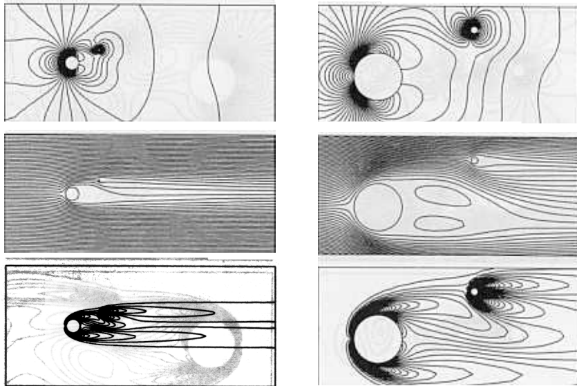
Figure 16. Re = 60 flow past main and control cylinders, P/D = 2 , T/D = pressure, streamfunction, and vorticity fields for the steady state solution.
