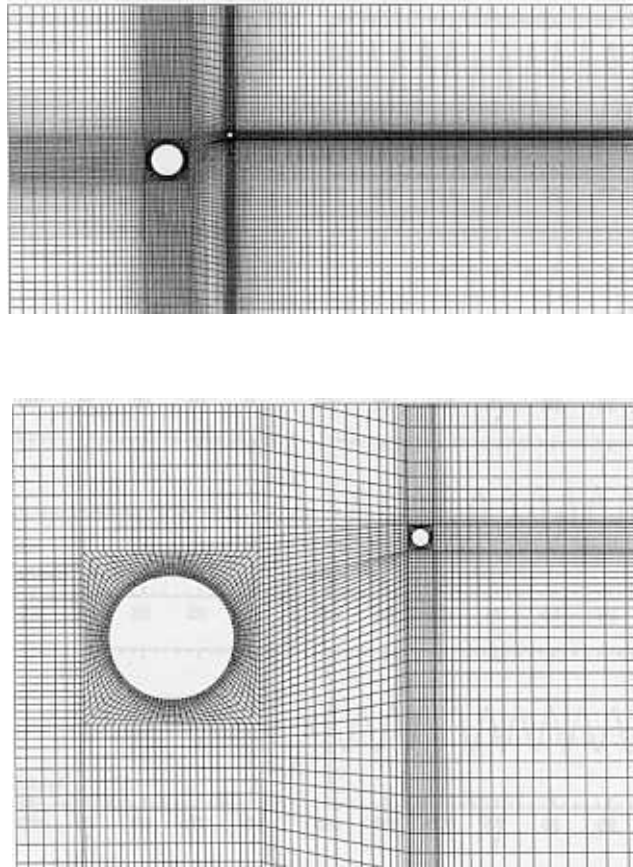
Figure 2. Flow past main and control cylinders, P/D = 2 , T/D = 0.8 : finite element mesh (and its close-up) with 10076 nodes and 9816 elements.
