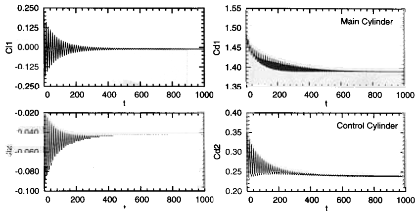
Figure 21. Re = 80 flow past main and control cylinders, P/D = 2 , T/D = 0.8 : time histories of the drag and lift coefficients for the main and control cylinders.
