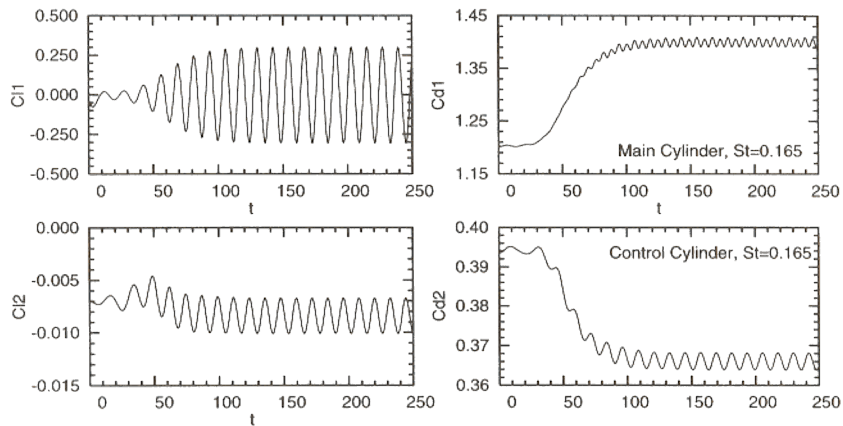
Figure 9. Re = 100 flow past main and control cylinders, P/D = 5 , T/D = 5 : time histories of the drag and lift coefficients for the main and control cylinders.
