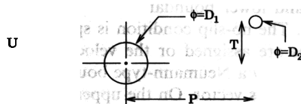
Figure Description of the relative location of the main and control cylinders.
