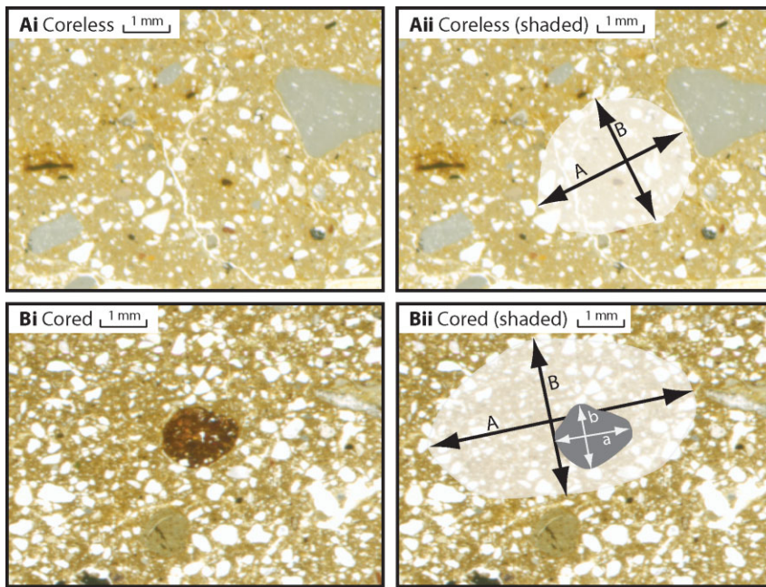
Fig. 1. Paired images of turbate microstructures in plane-polarized light showing coreless (Ai and Aii), and cored examples (Bi and Bii). Annotations indicate the manner in which the dimensions of the microstructures were measured. This figure is available in colour at http://www.boreas.dk .
