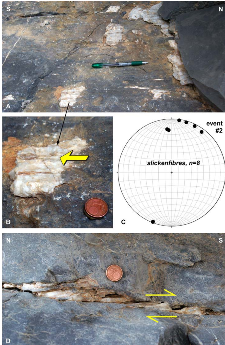
Fig. 6. Structures of event #2. (A) Slickenfibres on shallow-dipping veins indicating top-to-the-South sense of layer-parallel shearing in limestones. (B) Detail of photo (A). The diameter of the 1-cent Euro coin is 16.25 mm. (C) Summary of the orientations of slickenfibres on layer-parallel veins at the three localities where they were found. Each dot represents an individual measurement. Note that the original data have been rotated in this plot assuming that layers were horizontal when the structures developed. (D) Stepped layer-parallel vein showing top-to-South movement.
