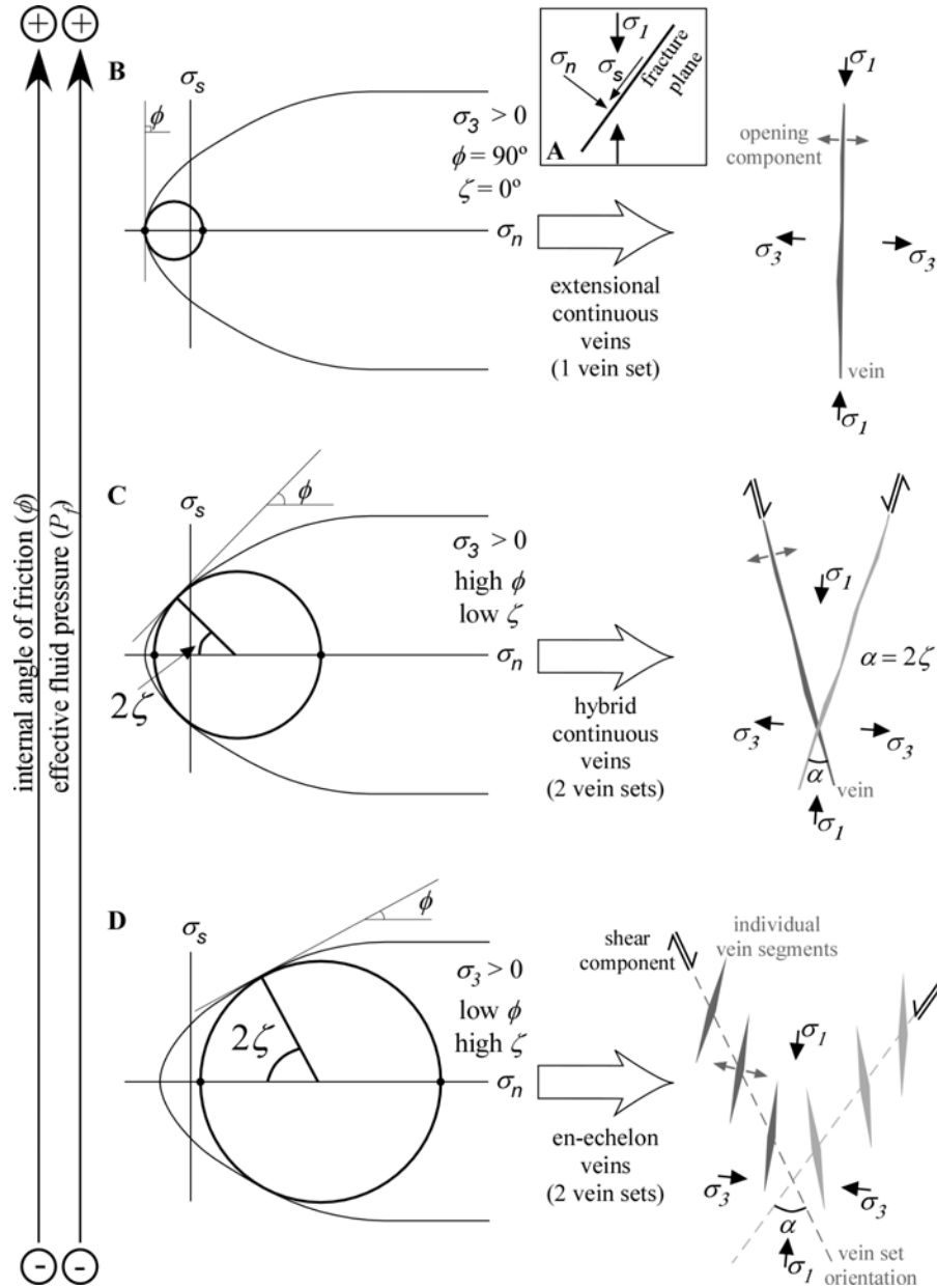
Fig. 14. Sketches and Mohr circles illustrating the effect of effective fluid pressure increase on the onset of fracture/vein sets. (A) Shows the definition of normal ( \sigma_n ) and shear ( \sigma_s ) stresses. An increase in effective fluid pressure (from (D) to (B)) shifts the Mohr circle to the left. This effect enhances failure and the onset of fractures with a higher angle of internal friction ( \phi ) and lower angle between conjugate sets ( \alpha ). (B) High fluid pressures lead to the onset of only one set parallel to \sigma_1 . (C) A relative high friction angle leads to two conjugate sets of hybrid fractures/veins with a significant opening component. (D) A smaller friction angle favors the onset of two conjugate sets of fractures/veins with a significant shear component. If these veins are segmented, individual segments have a significant opening component. Note that the angle \alpha is double in the Mohr circle ( \zeta ).
