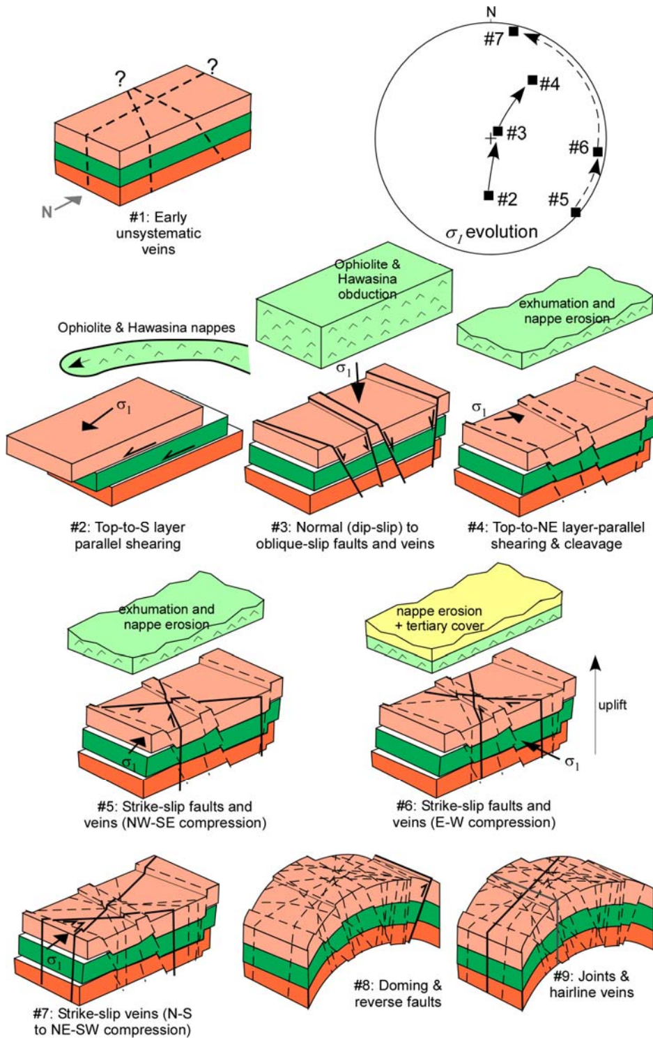
Fig. 13. Sketches summarizing the structural evolution of the Jabal Akhdar dome, with the order of identified events and calculated stress fields orientations. The stereogram illustrates the evolution of \sigma_1 showing two main trends: firstly obduction (#2), normal (dip-slip) and oblique-slip faulting (#3), reverse thrusting and exhumation (#4), and secondly a far horizontal \sigma_1 that comprises three events (#5 to #7). It is possible that event #3 did not form after obduction but before it.
