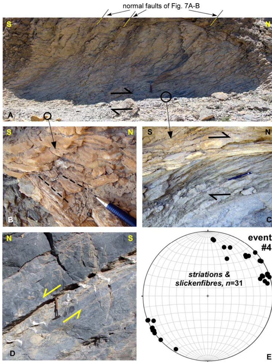
Fig. 9. Effects of event #4. (A) S-N view of top-the-Northeast shearing of the normal faults of figure 7A-B (Nahr Umr Fm). (B) Detail of layer-parallel striations pointing towards the Northeast. (C) Detail of top-to-the-northeast layer-parallel shearing. (D) Sigmoidal calcite veins sheared towards the NE (Shams Fm). (E) Summary of the orientations of striations and slickenfibres directions at the six localities where layer- and cleavage-parallel veins with a NE shearing direction were found (event #4). Each dot represents the average of measurements at each outcrop. Note that original orientations have been rotated in this plot considering that layers were horizontal when these structures were formed.
