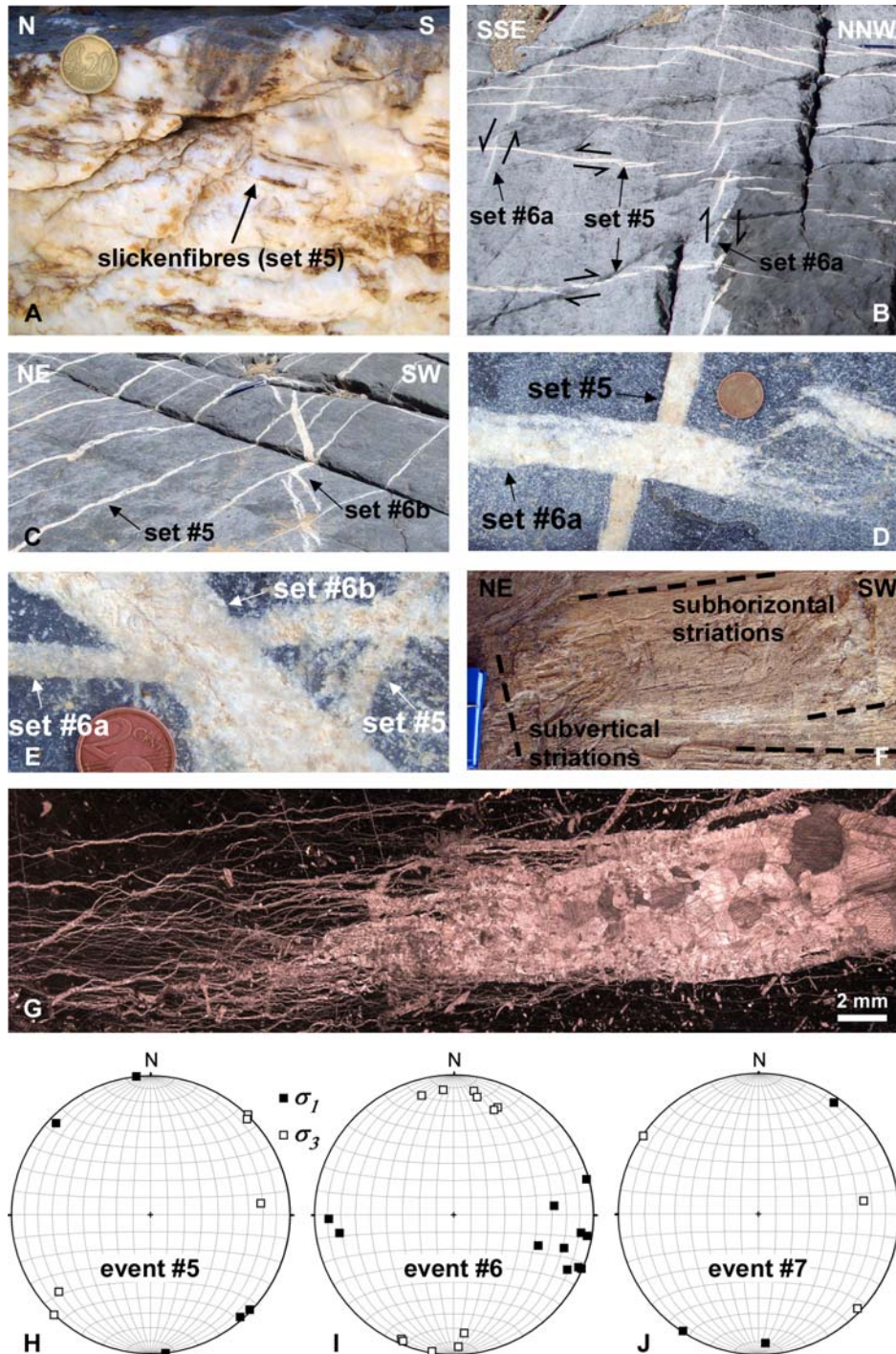
Fig. 10. (A) Vein of event #5 with subhorizontal slickenfibres crystals. (B) en-échelon conjugate sets of veins of event #6a (E-W-compression oriented) crosscutting veins of event #5 (NW-SE-compression oriented). (C) en-échelon veins of event #6b (NNE-SSW-oriented compression) crosscutting veins of event #5. (D-E) Examples of cross-cutting relationships between the different strike-slip vein sets. A stylolite dissolves the center of a vein of event #6b. (F) E-W-oriented large-scale fault with two sets of striations indicating older dip-slip and younger strike-slip movements. (G) Microphotograph showing the typical crack-seal microstructures of veins of the three strike-slip events. These veins are generally formed by hundreds or thousands of micro-crack events. This photo illustrates the transition from distributed to localized crack-sealing of a vein of event #6b. (H-I) Summary of the orientations of
