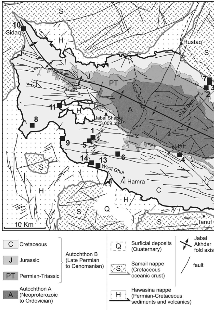
Fig. 3. Simplified map of the western part of the Jabal Akhdar dome. Squares with numbers indicate the location of the areas used for this study. Dashed lines are rivers or water streams that define wadis (valleys). A complete list of localities with coordinates is shown in table 1. Figure compiled from the Geological Map of Oman (Rustaq sheet), scale 1:100,000 (Beurrier and others, 1986). Locality 12 is out of the map. Thin lines indicate fault traces. The geographical coordinates of the upper left corner are (57°00'E, 23°30'N).
