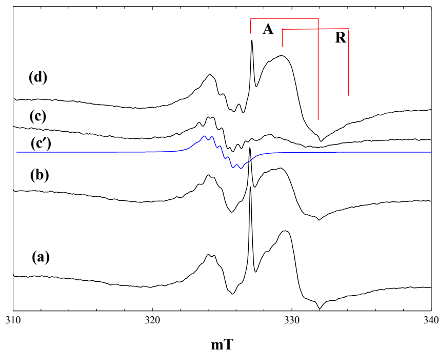
Figure 3. EPR spectra of P25 titania in a solution of phenoxyacetic acid in acetonitrile at 4 K. (a), During irradiation with low intensity 400 nm light; (b), During irradiation with high intensity 400 nm light; (c), during irradiation with high intensity broad band light; (d), after stopping irradiation; (c'), a simulated spectrum of the phenoxyacetic acid radical cation, as described in the text.
