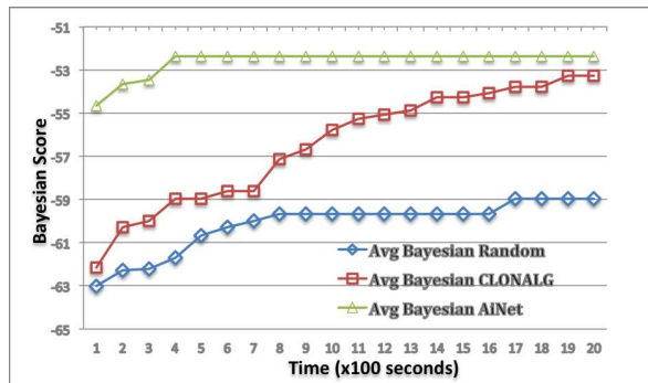
Fig. 5. Experimental Results for MG-7Hid: Average Bayesian Score of the Best Candidate Model Over Ten Trials
