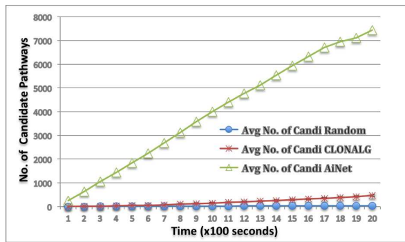
Fig. 4. Experimental Results for MG-7Hid: Average Number of Candidate Models Found Over Ten Trials
