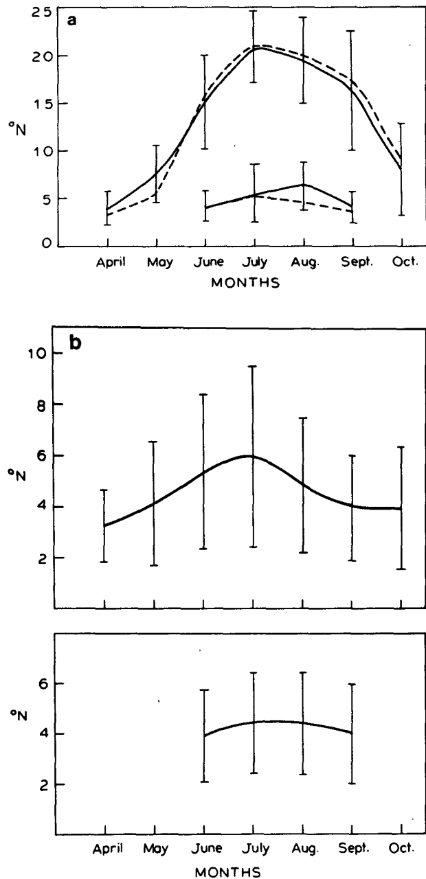
FIG. 3. (a) Monthly mean location of the axes of the northern and southern MCZ (solid line, 90°E; dashed line, 80°E). The standard deviation at 90°E is also shown. (b) Monthly mean width of the northern (top) and southern MCZ's at 90°E. The standard deviation is also shown.
