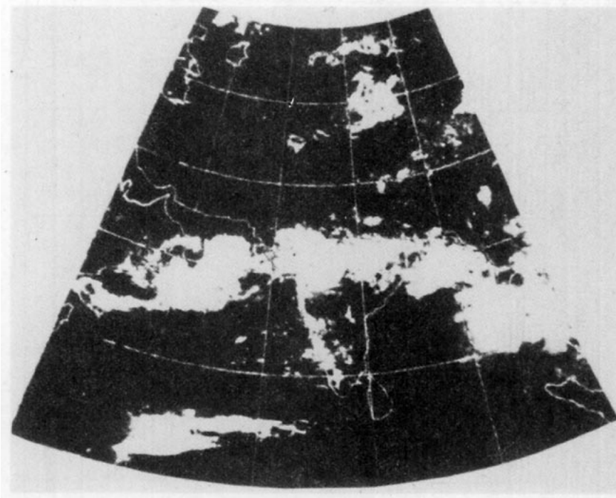
FIG. 1. The MCZ on 8 July 1973.
