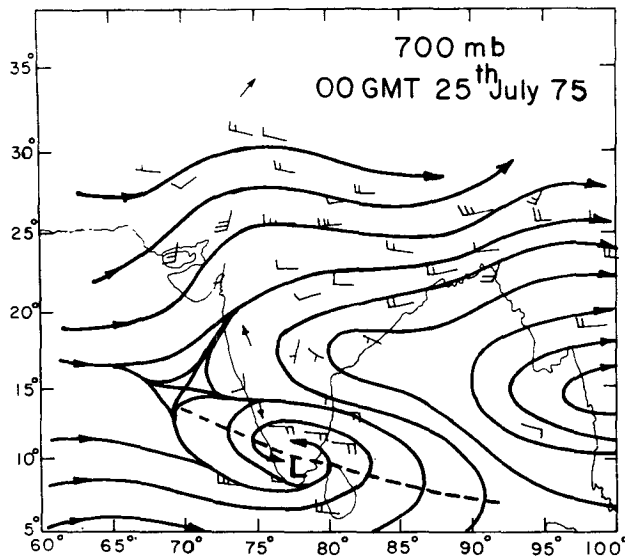
FIG. 8. Streamlines at 700 mb for 25 July, 31 July and 6 August 1975 at 0000 GMT.
