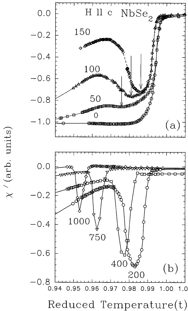
FIG. 1. Temperature variation of the in-phase ac [ f = 21 Hz, h_{ac} = 2 Oe (rms)] susceptibility \chi'_H(T) for H||c in a single crystal of 2H\text{-NbSe}_2 [ T_c(0) \approx 7.1 K]. The arrows identify the positions ( T_{\text{peak}}(H) ) of negative peak in \chi''(T) plots.
