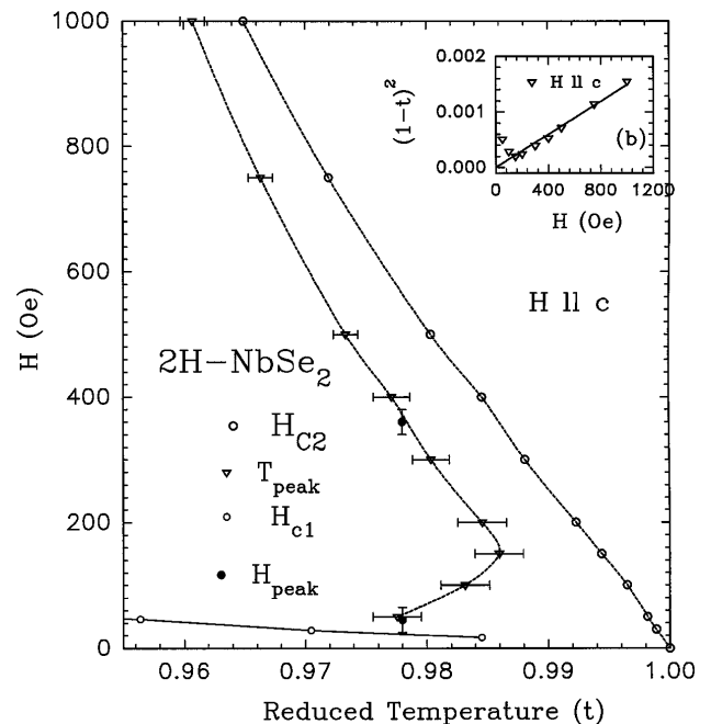
FIG. 2. Magnetic phase diagram near T_c(0) in the 2H\text{-NbSe}_2 system. The inset shows the variation of [1 - T_{\text{peak}}(H)/T_c(0)]^2 with field for H||c .
