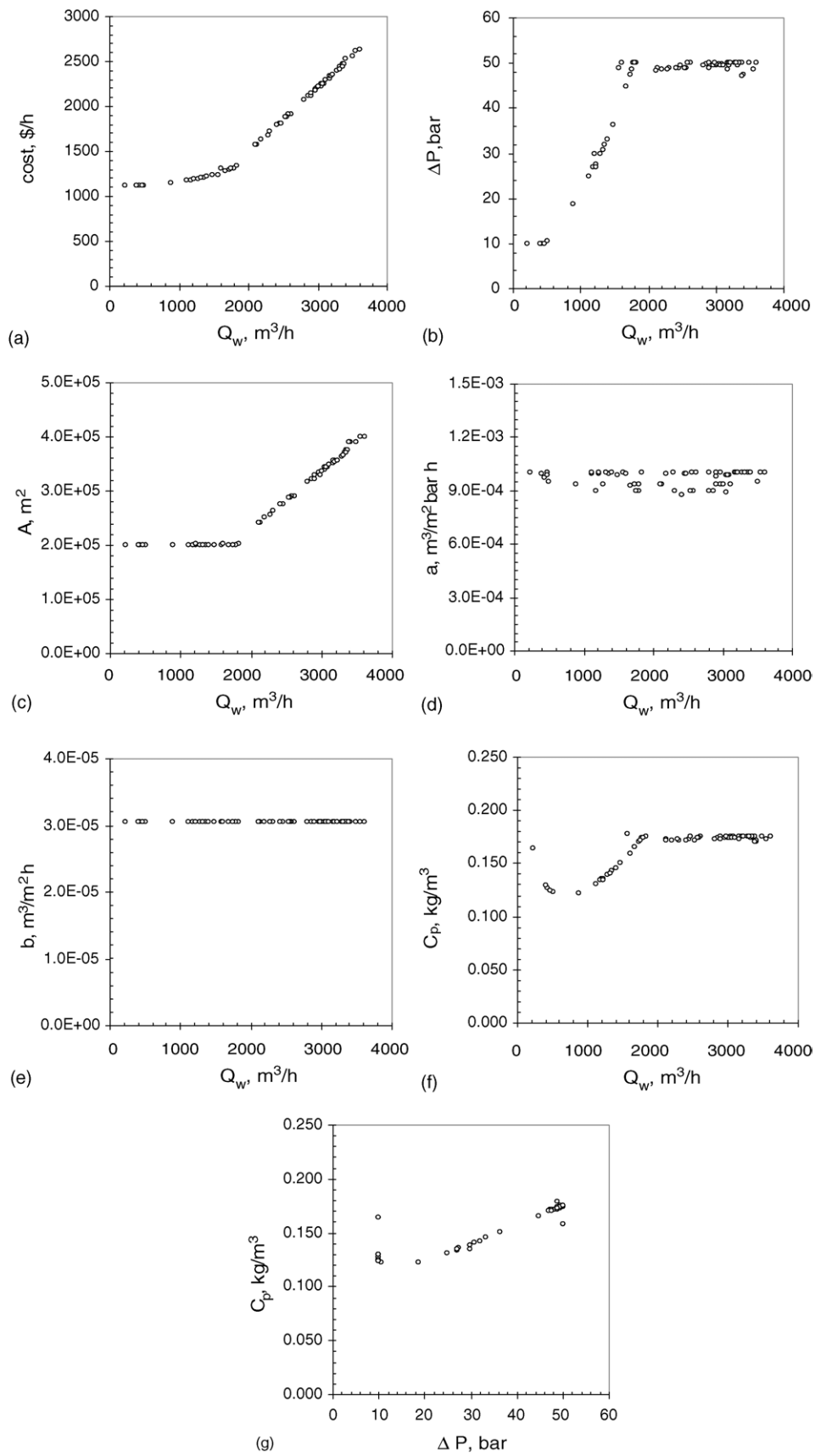
Fig. 2. Optimal solutions for Problem 3 (see Table 1 for details).
