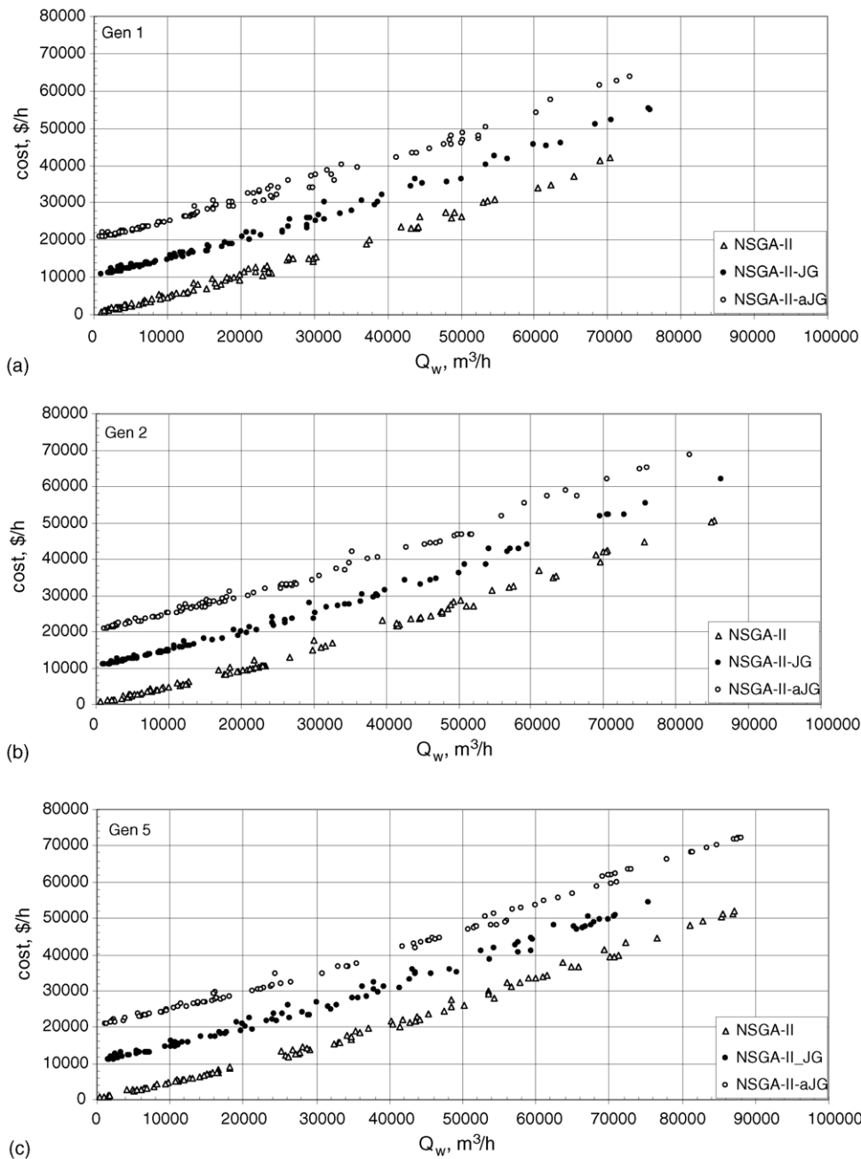
Fig. 5. Optimal Pareto solutions for Problem 4 using NSGA-II, NSGA-II-JG and NSGA-II-aJG (results for NSGA-II-JG and NSGA-II-aJG are displaced upwards by 10,000 and 20,000 $ h -1 , respectively, on the ordinate so that the plots can be easily compared).
