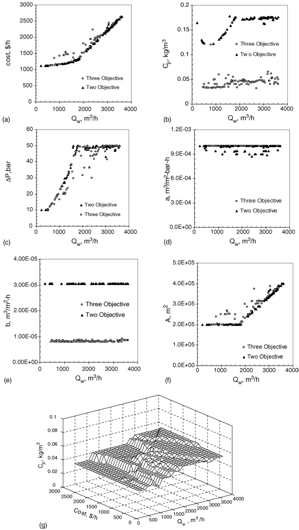
Fig. 4. Optimal solutions for Problem 5 (see Table 1 for details).
