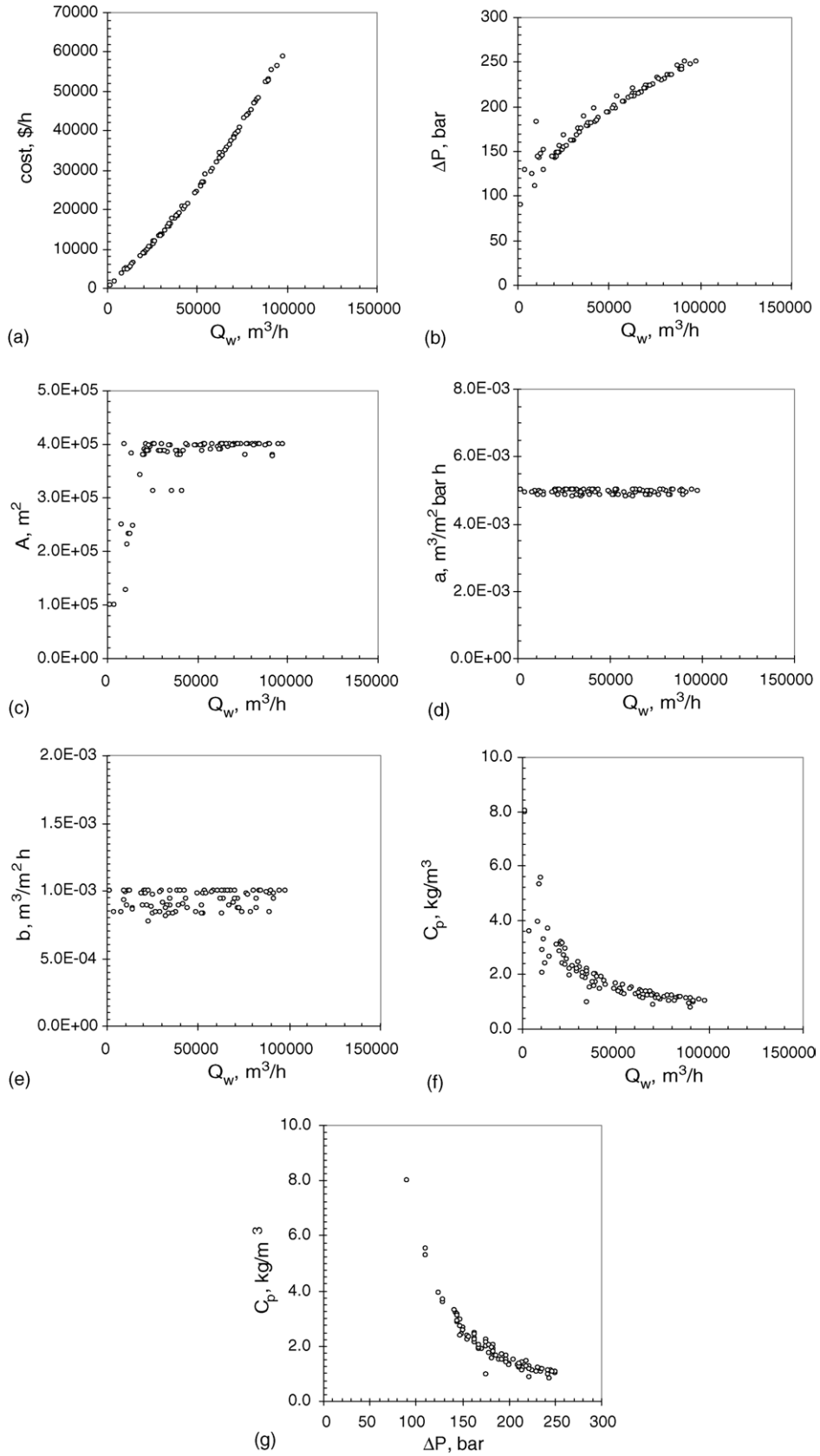
Fig. 3. Optimal solutions for Problem 4 (see Table 1 for details).
