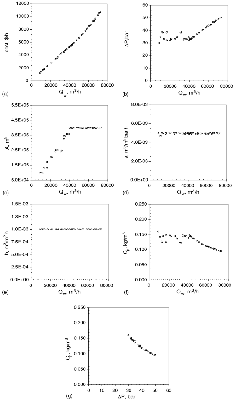
Fig. 1. Optimal solutions for Problem 2 (see Table 1 for details).
