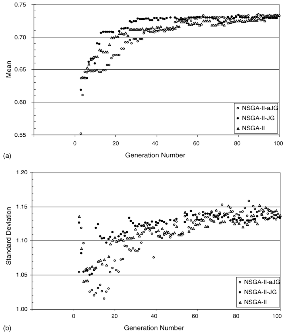
Fig. 6. Mean and standard deviation of I_{i,dist} for the Pareto solutions (shown in Fig. 5) of Problem 4 (for N_{gen} \geq 3 ).
