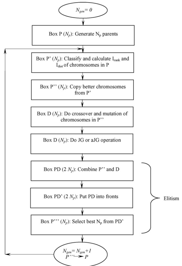
Fig. A1. Flow chart of NSGA-II and the JG adaptations.
