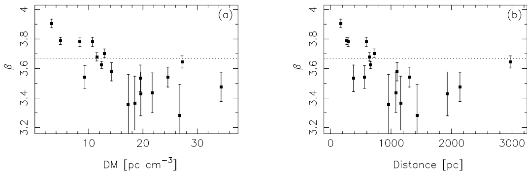
FIG. 3.—Values of \beta are plotted against (a) DM and (b) distance. For PSR B0823+26, PSR B0834+06, PSR B1133+16, and PSR B1919+21, \langle\beta\rangle (the average of \beta from different observing sessions) is used. The dotted line indicates the Kolmogorov index 11/3. The uncertainties in values of \beta are at \pm 1 \sigma levels.
