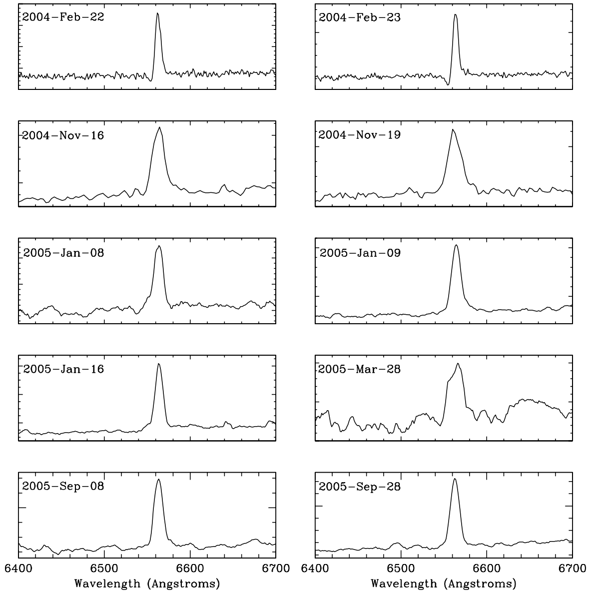
Figure 8. The H \alpha profiles of V1647 Ori seen in the spectra obtained with HFOSC between 2004 February 22 and 2005 September 28. The H \alpha line shows a pronounced blue-shifted P Cygni profile in the spectra taken in the early phase of outburst (2004 February 22 and 23).
