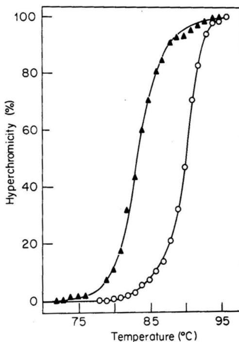
Figure 1. Thermal denaturation of DNA. Native DNA in 0.12M sodium phosphate buffer, pH 6.8, was melted at 1°C increments in a Gilford Spectrophotometer 250 equipped with a thermoprogrammer (model 2527). Escherichia coli DNA was used as standard. The DNA melting temperature ( T_m ) and G+C content were calculated according to Mandel and Marmur (1968). The open circles represent E. coli DNA and the closed triangles, DNA from mealybug (gravid females).
