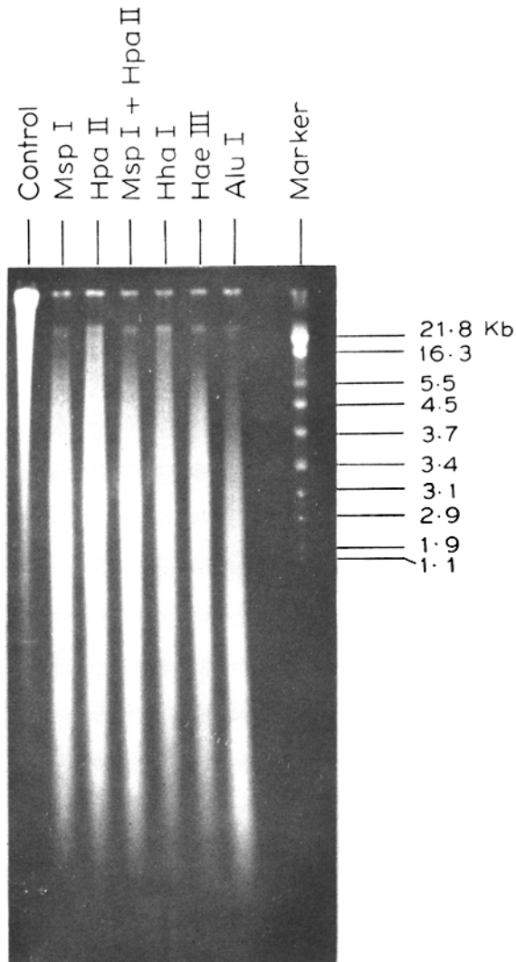
Figure 2. Restriction enzyme digestion of DNA. Two \mu\text{g} of mealybug DNA was digested for 6 h at 37°C with 4 units of the enzyme. DNA fragments were separated by electrophoresis at 50 volts for 8 h on 1% agarose gel. \lambda DNA digested with EcoRI and Bam HI was used as molecular weight marker.
