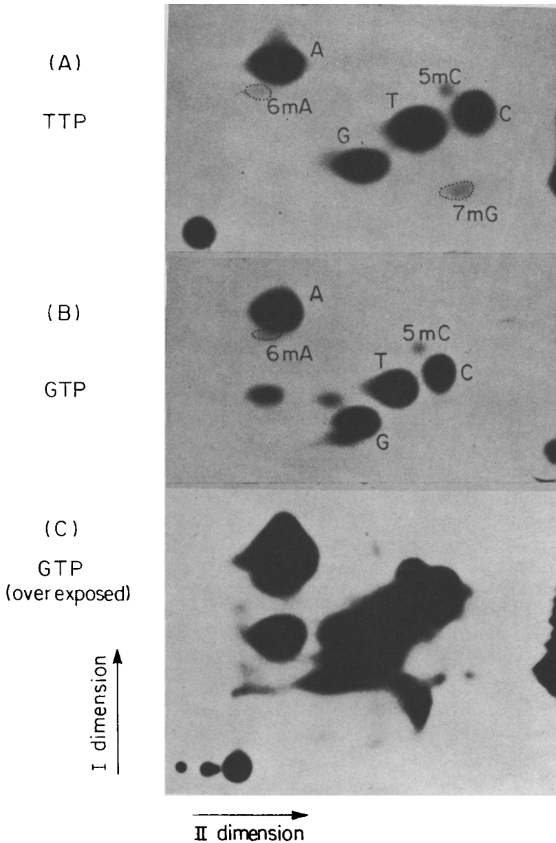
Figure 3. Dinucleotide analysis. 3' \alpha - ^{32}\text{P} labelled nucleotide monophosphates were chromatographed under the same conditions as those employed for separation of the Standard dNMPs (figure 4).
