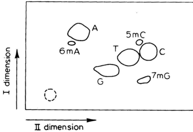
Figure 4. Separation of deoxynucleotide monophosphates on two dimensional TLC. Diagrammatic representation of observed separation of standard dNMPs following chromatography on cellulose TLC plates using Isobutyric acid: water: \text{NH}_4\text{OH} (66:20: 1, v/v) in the first dimension and saturated (\text{NH}_4)_2\text{SO}_4 in the second dimension.
