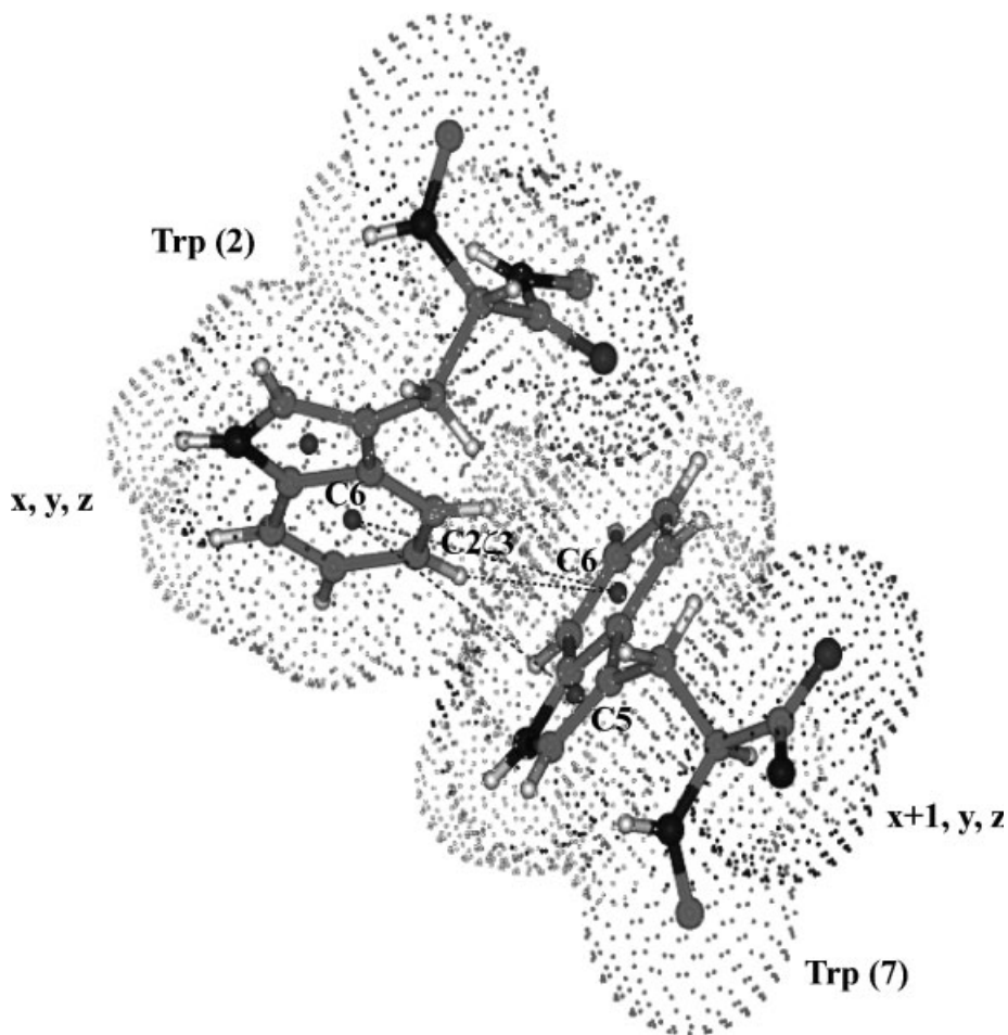
Figure 13. Close packing of the two Trp rings observed in the crystals of peptide 1 (the van der Waals surfaces are shown). The parameters defining aromatic interactions are: R_{6cen} = C6...C6 = 5.72 \text{ \AA} ; R_{5cen} = C5...C5 = 6.77 \text{ \AA} ; R_{6,5cen} = C6...C5 = 4.87 \text{ \AA} ; interplanar angle \{\gamma\} = 70.5^\circ ; C2\zeta_3...C6 = 4.41 \text{ \AA} ; H2\zeta_3...C6 = 3.51 \text{ \AA} ; \angle CH... \pi = 163.8^\circ .
