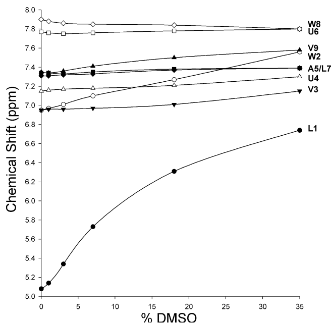
Figure 7. Chemical shift variation of backbone NH resonances in peptide 2 , in \text{CDCl}_3 , with increasing dimethyl sulfoxide (DMSO) concentration. The amide resonances of residues 1 and 2 show a strong solvent dependence (peptide concentration: 10 mg/mL).
