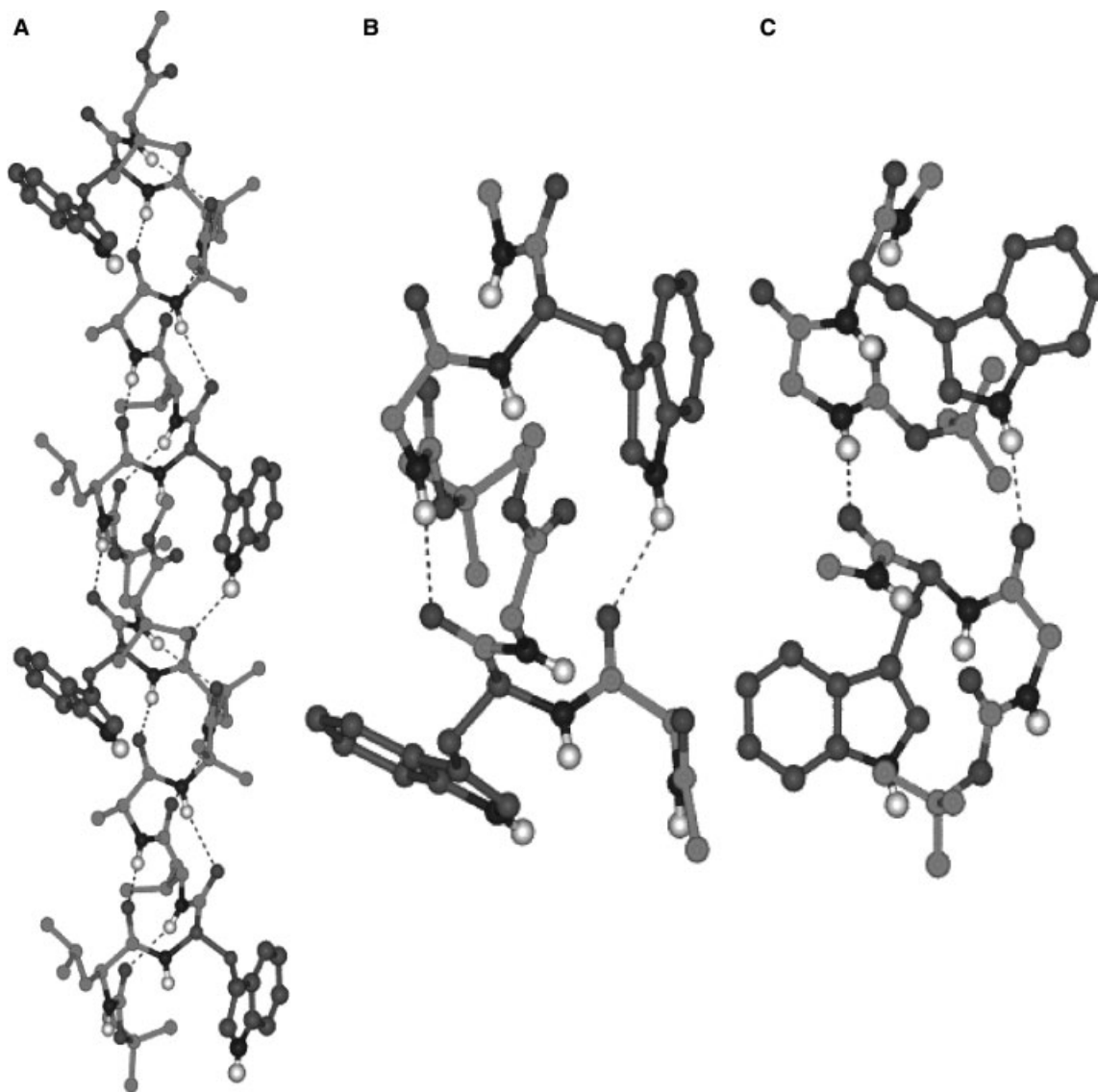
Figure 12. (A) View of the helical column of peptide 1 stabilized by intermolecular hydrogen bonds [Trp(2)N \epsilon 1H...OCLeu(6) and Leu(1)-NH...OCTrp(7)]. (B) An expanded view of the stabilizing intermolecular hydrogen bonding interactions driving the packing of molecules in the crystals of peptide 1 , compared with that observed in peptide 4 (C).
