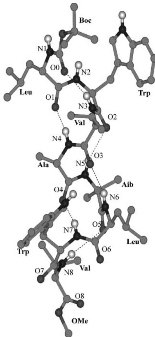
Figure 10. Molecular conformation of Boc-Leu-Trp-Val-Ala-Aib-Leu-Trp-Val-OMe, 1 , in crystals. The intramolecular hydrogen bonds are shown by dotted lines.
