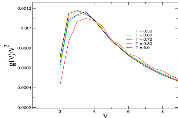
FIG. 10: Temperature dependence of the Boson Peak. The data is shown for S = 0.10 for different temperatures of the parent liquid.
