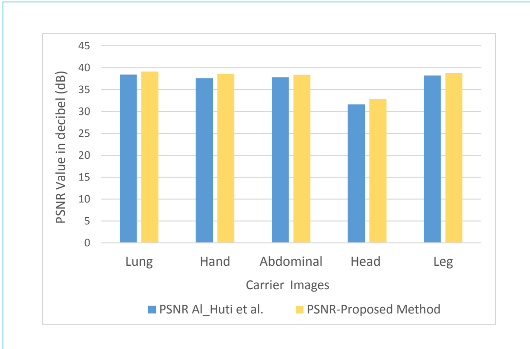
Figure 4.11 Variation of PSNR after concealing 196508 bits in medical cover images (corresponding stego images), which means that there is a high similarity between the stego image and the original cover image. Such degree of similarity can also be revealed by the image pixel values' average (Im_Pix_Avg). For example, the Im_Pix_Avg (136.3565) for Elaine cover image and the one for Elaine stego image (136.5613 ) as provided in Fig 4.9, they are very close to each other with the only difference of 0.2048 which is actually acceptable.
