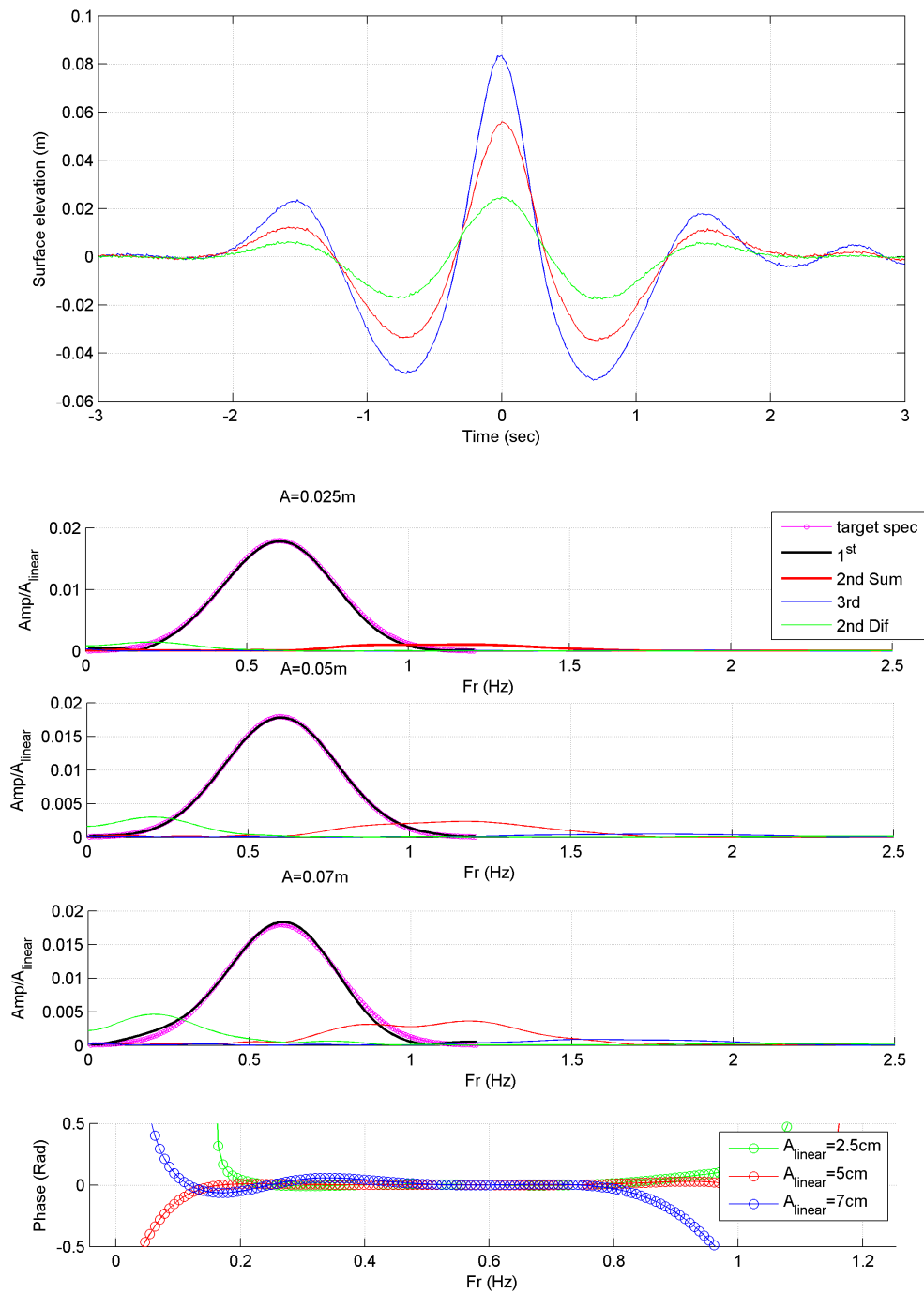
Figure 5: Starting from the top, measured surface elevation, spectra and phases at focus for A_{\text{linear}}=0.025\text{m} (green line), A_{\text{linear}}=0.05\text{m} (red line) and A_{\text{linear}}=0.07\text{m} (blue line). The focused waves illustrated were propagated on an in-line shear current with a surface flow velocity of 0.2m/s, see also Fig. 2.
