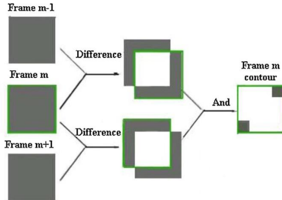
Gambar 2.1 Efek dari overlap -nya three-frame difference .
