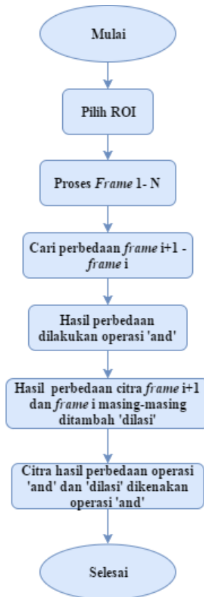
Gambar 4.11 Diagram alir Improved Three Frame Difference .
