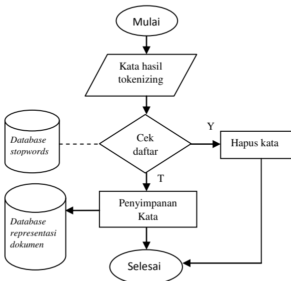
Gambar 4. 3 Diagram Alir Filtering
