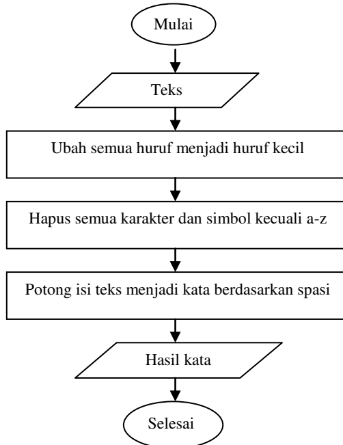
Gambar 4. 2 Diagram Alir Case Folding dan Tokenizing
