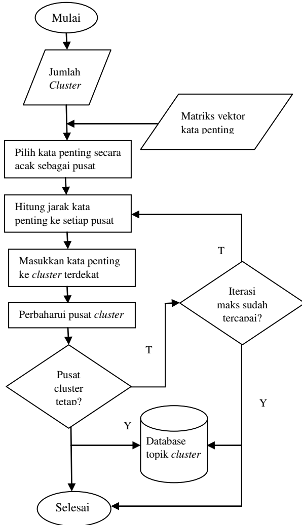
Gambar 4. 5 Diagram Alir K-Means Clustering
