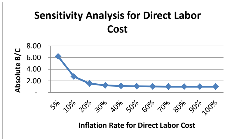
Figure 4. 12 Sensitivity Analysis for Direct Labor Cost
