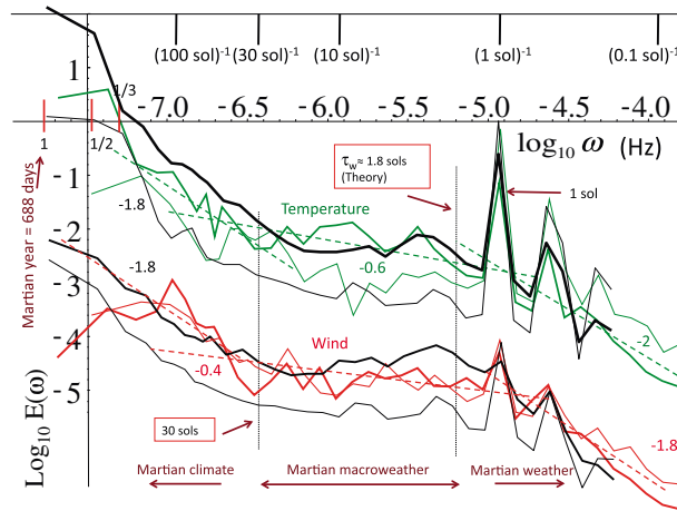
Figure 1. The Viking 1 and 2 (thin: 22°N, thick: 48°N) temperature and wind spectra (green and red) averaged over 10 bins per order of magnitude (logarithmically spaced); the units are K^2 h and m^2 s^{-2} h , respectively; the wind spectra have been displaced downward by 2 orders of magnitude for clarity. The pairs of black lines are from the reanalyses at corresponding latitudes (thin: 20°N, thick: 50°N). The data series were cubically detrended to remove much of the annual cycle. The three red ticks at the far left indicate the Martian year and harmonics at a half and a third of a year; these are the only frequencies significantly affected by the detrending. The dashed reference lines are the terrestrial values with slopes indicated [Lovejoy and Schertzer, 2013, chapters 8 and 10]. Also indicated are the three scaling regimes; the climate regime (below about (30 \text{ days})^{-1} ) is not clear since the spectrum rises due to the poorly resolved annual cycle.
