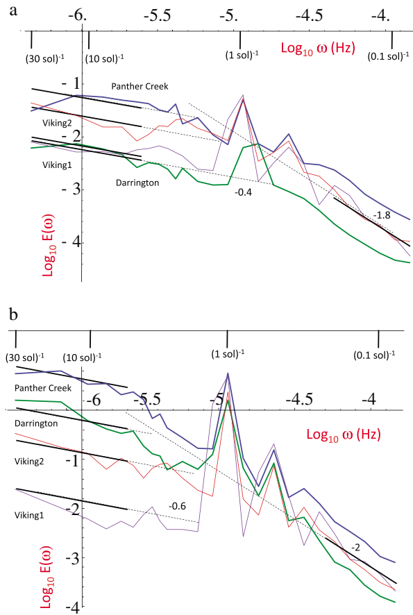
Figure 3. (a) Spectra for Earth and Martian surface temperatures from Panther Creek, Texas (blue), Darrington, Washington (green), Viking 1 (purple), and Viking 2 (red). The Earth stations have been offset (upward) by 1 order of magnitude for clarity. The reference lines have slopes -0.4 (low frequencies) and -1.8 (high frequencies). The units are K^2 h . To quantify the series to series spread/error, each of these frequency bin-averaged spectra was used to determine the standard deviations of the \log_{10} spectral densities about the means. At the low frequencies the variations were between \pm 0.6 and \pm 0.8 , whereas at the highest frequencies the variations were between \pm 0.2 and \pm 0.4 (decreasing roughly linearly from the low frequencies; the higher latitudes had the higher spreads). (b) The same as Figure 3a except for the wind data. The Earth stations have been offset (upward) by 1 order of magnitude for clarity. The reference lines have slopes -0.6 (low frequencies) and -2 (high frequencies). The units are K^2 m^2 s^{-2} . The spreads of the individual spectra about the means were close to those of the temperatures in Figure 3a.
