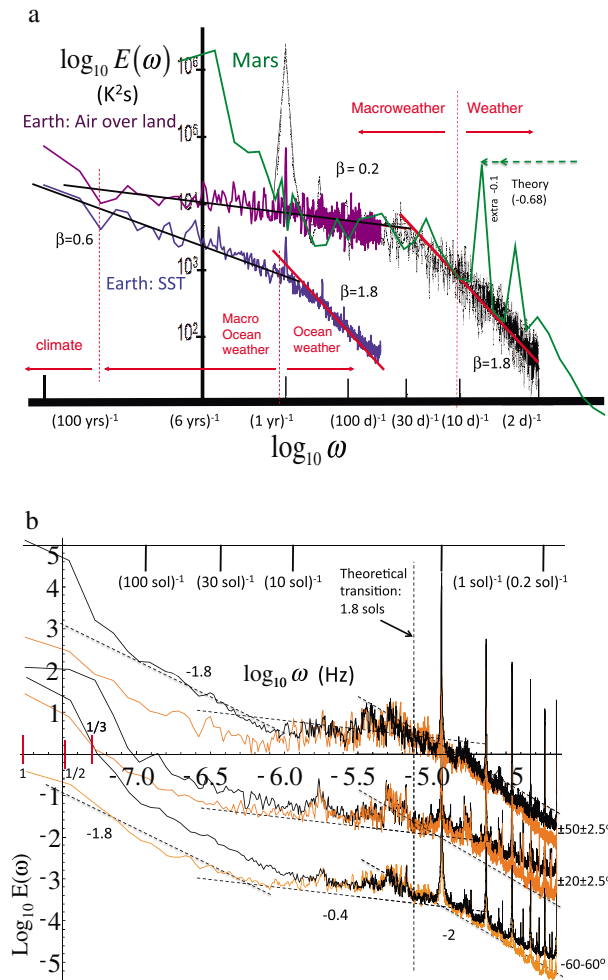
Figure 2. (a) A comparison of the Martian temperature spectrum (cubically detrended, green, from Viking 2 (Figure 1), shifted left by the theoretical amount ( -0.68 ) and an additional 0.1 for a better fit), superposed on an Earth air over land spectrum (monthly data, 100 years long, purple, left) and sea surface temperature (SST, blue, bottom left). Also shown (right, black, reproduced from Lovejoy and Schertzer [1986]) is the spectrum of daily temperatures from Macon France. The red reference lines have slopes -1.8 . The weather, macroweather regimes are indicated; the climate regime (frequencies < \approx (50 \text{ years})^{-1} ) is only hinted here (see Lovejoy and Schertzer [2013] for a discussion and review of this and other evidence). Adapted from Lovejoy and Schertzer [2012, Figure 4]. (b) Martian reanalysis: 660 sols of data sampled every 1/12 sol, starting at year 24 longitude 141^\circ , (May 1999) sigma level 0.995 (near surface). Black is temperature; orange is the zonal wind, units: K^2 h and (m/s)^2 h . The dashed vertical line is the theoretical weather/macroweather transition. The 20^\circ latitude pair has been shifted upward by 2 orders of magnitude, the 50^\circ latitude by 4 orders. The bottom pair is for the entire planet between \pm 60^\circ latitude. The dashed lines have reference slopes as indicated. Red lines indicate Martian year and fractions thereof. To quantify the series to series spread/error, each individual spectrum was averaged over logarithmically spaced frequency bins as in Figure 3. The standard deviations of the \log_{10} of the bin- (frequency range) averaged spectra were found to decrease roughly linearly from \pm 0.8 to \pm 0.4 from low to high frequency ( \pm 60^\circ curves), from \pm 0.7 to \pm 0.2 ( 50^\circ curves), and \pm 0.6 to \pm 0.2 for ( 20^\circ curves), with very similar spreads for temperature and wind.
