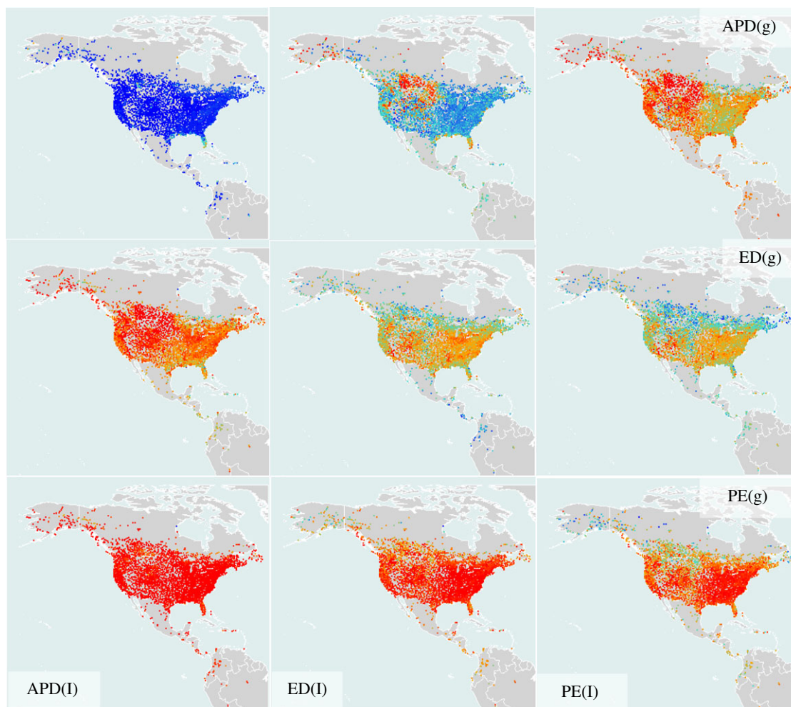
Figure 2. Map of correlations between local evolutionary isolation scores (I) and global evolutionary isolation scores (g) for 4628 bird communities for three different measures of evolutionary isolation—descriptions in text. Blue colours are higher correlation (light blue is a coefficient of approximately 0.7; dark blue represents a value tending to 1), orange-red colours show weaker correlation (red represents a correlation coefficient of 0 to around 0.4; orange around 0.55). (Online version in colour.)
