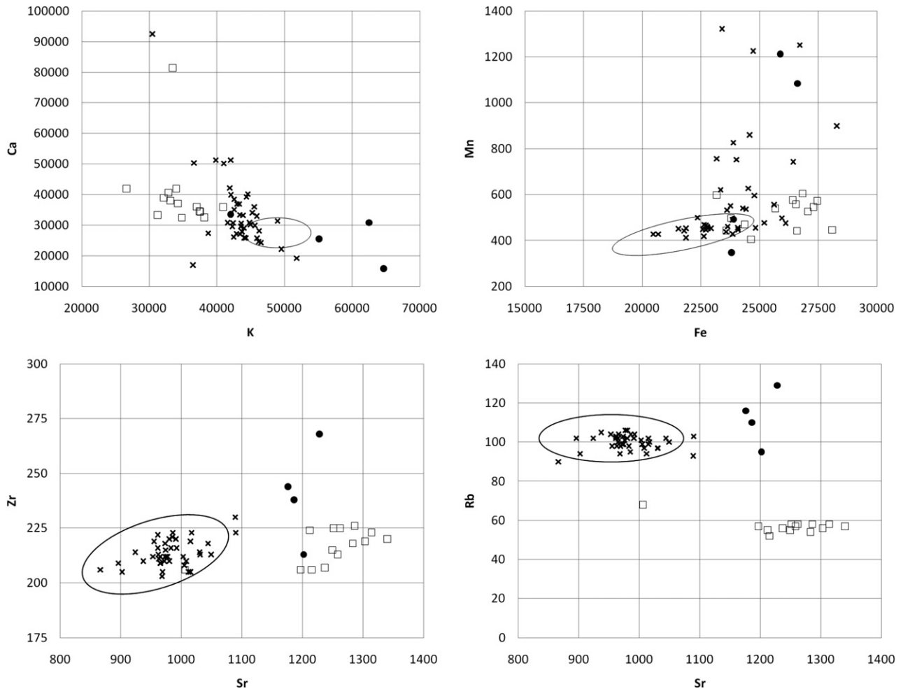
Fig. 4. Bi-variate plots of K vs. Ca, Fe vs. Mn, Sr vs. Zr, and Sr vs. Rb (in ppm) for andesite building stones from the Cuzco region, including stones assigned to the Rumiqolqa quarry (x) and the unidentified andesite X (open squares) and Y (filled circles) sources; the oval indicates the range of variation of fresh surfaces of Rumiqolqa quarry samples; error bars are not included because they would have been smaller than the individual points.
