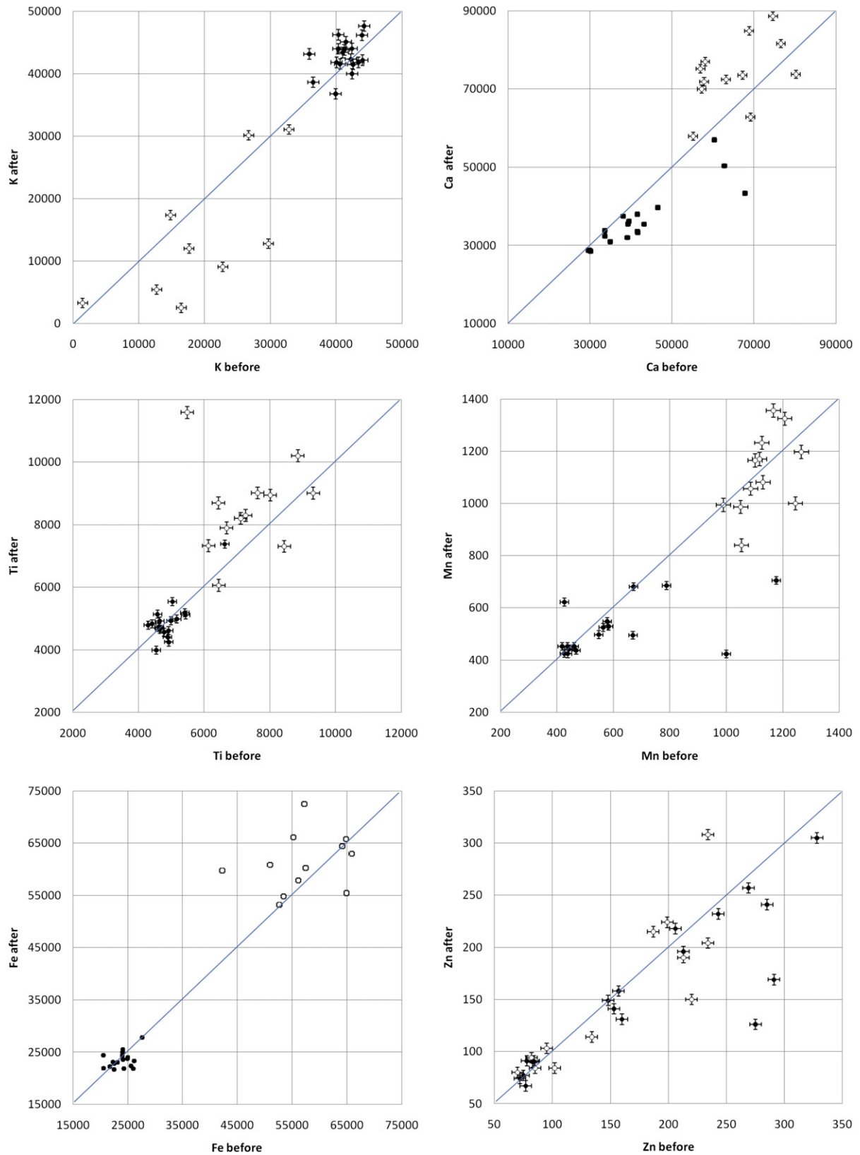
Fig. 3. Paired measurements of concentrations of elements (in ppm) before (X axis) and after (Y axis) cleaning surfaces of the same building stone, including Rumicolqa andesite blocks (solid circles) and diorite (open circles); error bars represent instrument counting error at one standard deviation.
