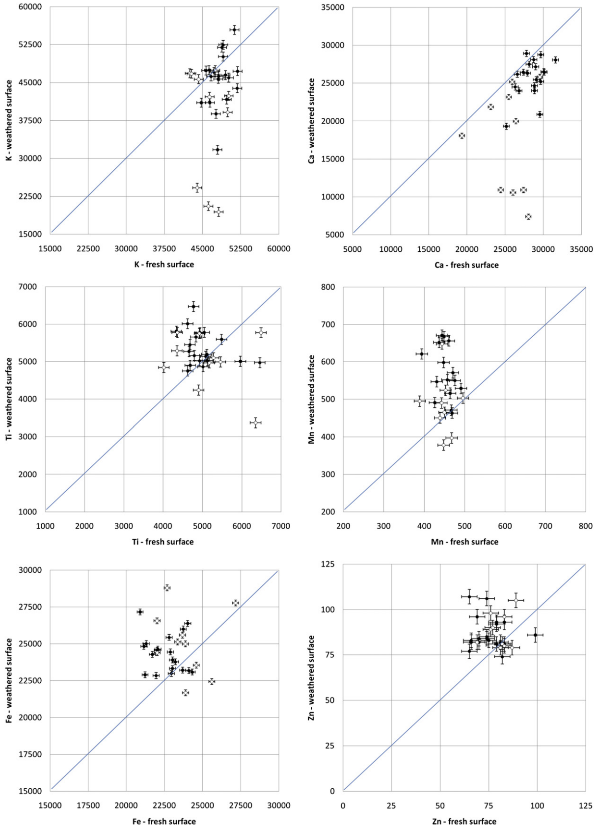
Fig. 2. Paired measurements of concentrations of elements (in ppm) from fresh (X axis) vs. weathered (Y axis) surfaces of the same sample, comparing Rumiqolqa (solid circles) and Huaccoto (open circles) andesites; error bars represent instrument counting error at one standard deviation.
