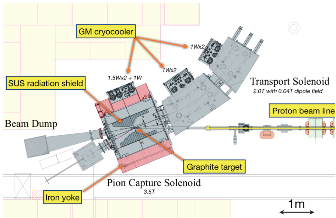
Figure 2.3: Schematic of the current status of MuSIC. Taken from [11]
