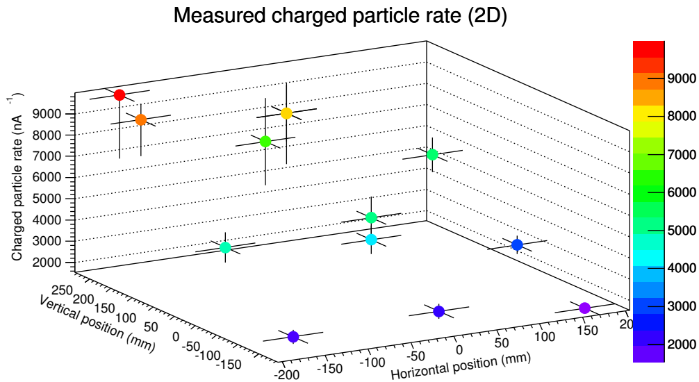
Figure 4.7: 2D plot of the charged particle flux across the front of the MuSIC beam pipe. The final three measurements were rescaled using the ratio of the two measurements at (0, 20) cm. Both the dot colour and the z-axis indicate the flux.
