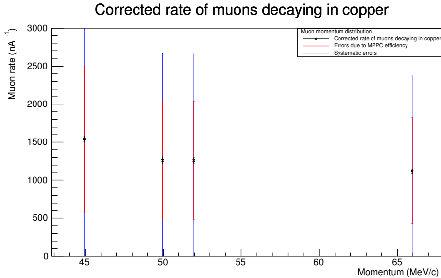
Figure 4.26: Corrected decay rate of muonic copper. The simulated rates are not shown as the statistics for muonic copper decays were too low to extract reasonable values from. The blue line indicates the error due to systematic error, the red line is the MPPC efficiency error and the black line the statistical error.
