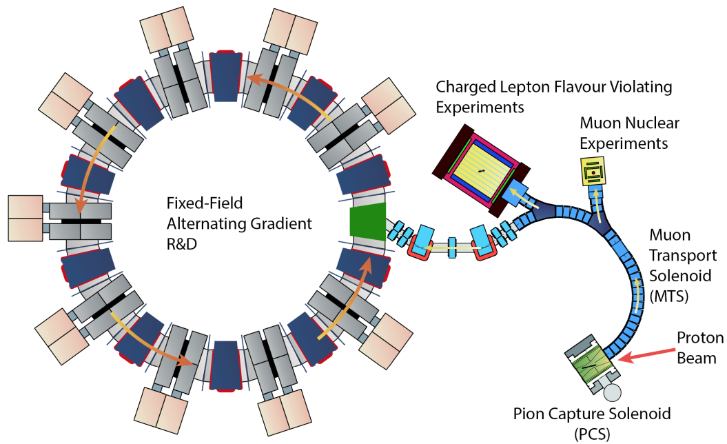
Figure 2.2: Schematic of the completed MuSIC complex. Taken from [1].
