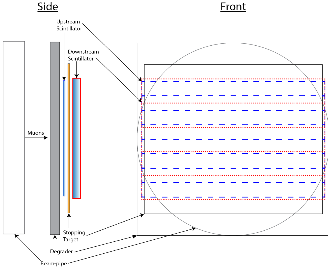
Figure 3.6: Schematic of the detector configuration for simulation. In the face on view the dotted lines are the scintillators, blue for the eight upstream scintillators and red for the five downstream scintillators.
