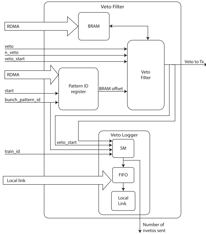
Figure 7.5: Block diagram of the veto filter. Note: veto_start is the start signal synchronised to the vetos, start is the START signal from the Rx block and used to load the bunch pattern.
