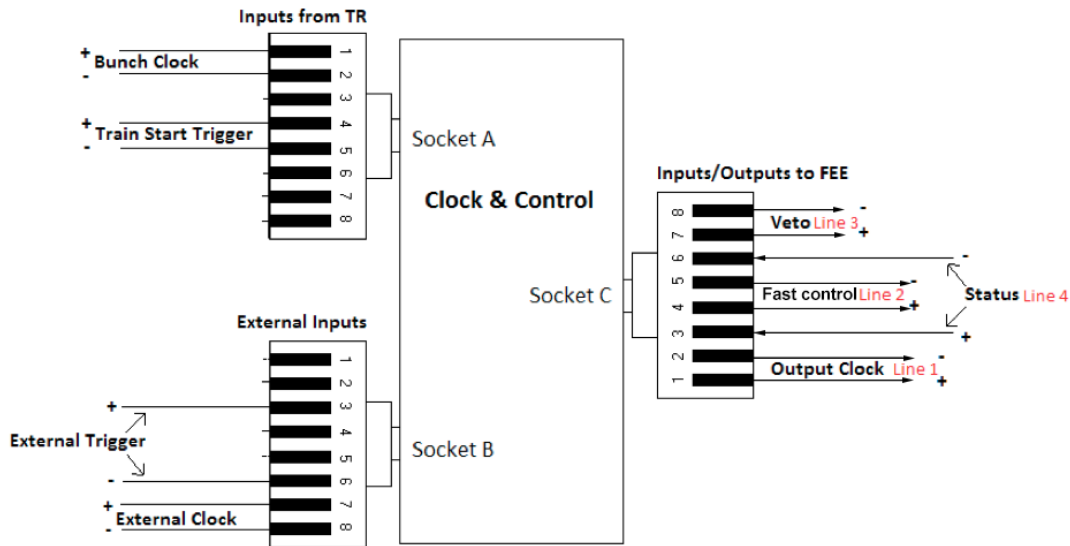
Figure 5.3: The CCC RJ45 wiring diagram. Arrows on the inputs/outputs to FEE indicate signal direction, apart from the status line all are input to the FEE, i.e. the status line is the only line expected to send signals from the FEE to the CCC. Modified from [31].
