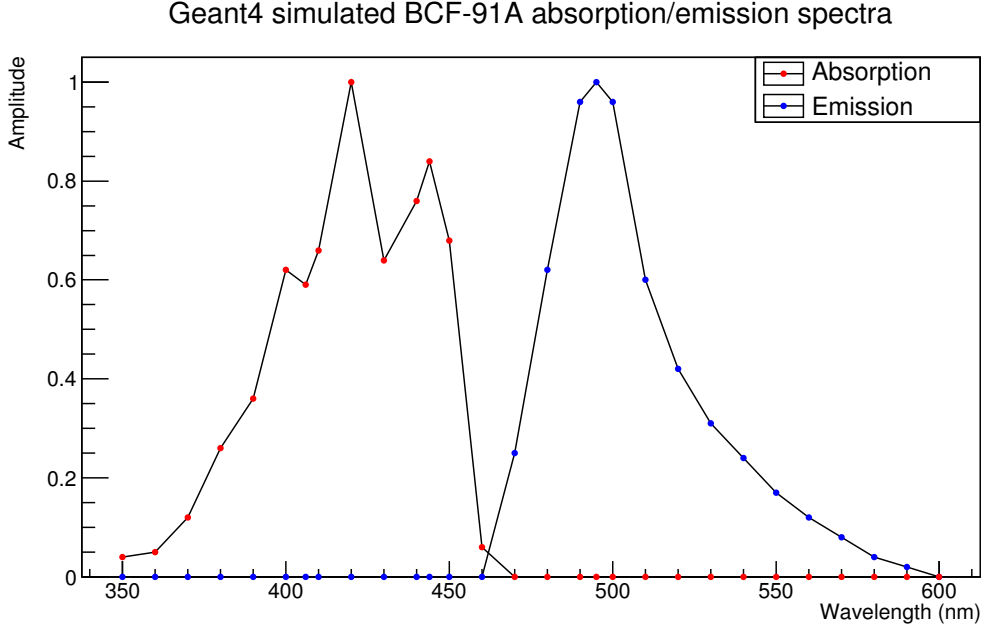
Figure 3.9: Absorption and re-emission spectra for BCF-91A wavelength-shifting fibre. The points represent the values used in Geant4 to approximate the manufacturer’s curve as given in the data-sheet [28].
