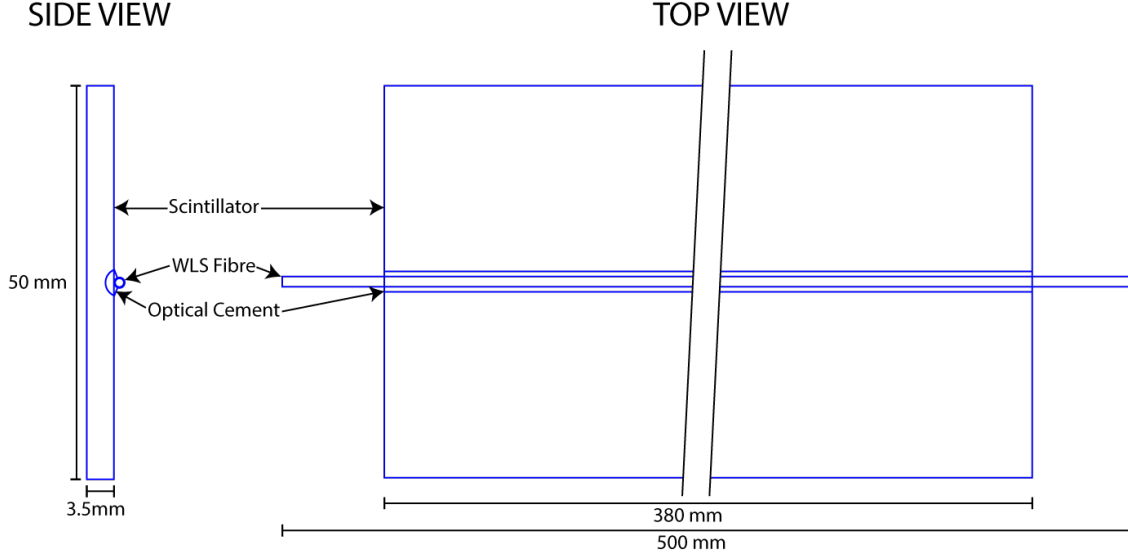
Figure 3.7: Schematic of a downstream paddle. The upstream paddles have the same layout but are have a different width and height (0.5 mm and 30 mm respectively). The WLS fibre protrudes from the scintillator for easy attachment of the MPFCs to the support structure.
