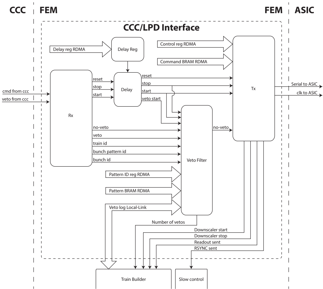
Figure 7.1: Top level block diagram. The clk and rst signals are supplied to each block and have been excluded from block diagrams unless otherwise noted. clk can either be an internal signal if the board is running in a standalone mode or is the clock received from the CCC. rst is an internal board reset, not to be confused with the RESET command which is intended to reset the ASIC (not the FEE).
