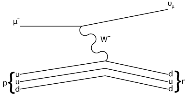
Figure 2.8: Nuclear capture of a negative muon. This process is very hard to detect directly. The net effect is to reduce the muon’s apparent lifetime by removing them from the population.
