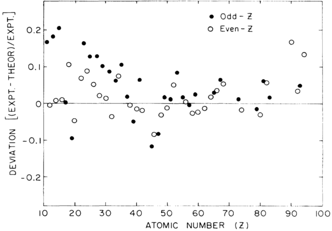
Figure 2.9: Comparison of the theoretical values (as determined using the Primakoff-Goulard formula) and experimentally determined muon capture rates for a range of materials, taken from [3].
