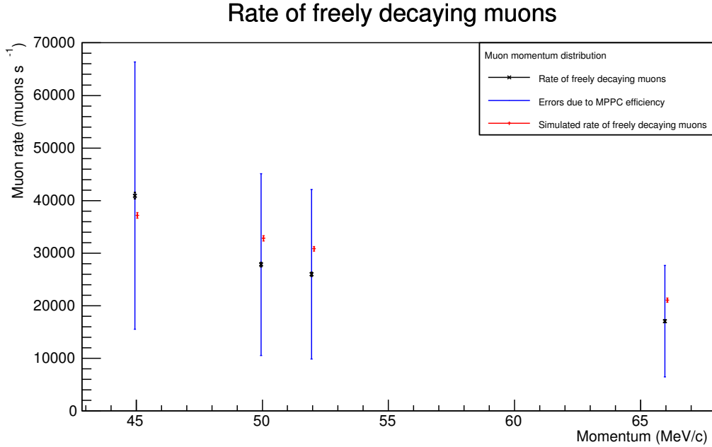
Figure 1.1: Measured muon momentum spectrum for freely decaying muons at MuSIC. The muon rate is normalised to a proton beam current of 1 nA.
