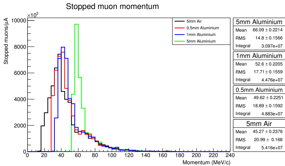
Figure 4.14: Momenta at the end of the beam pipe of muons that subsequently stopped. A stopped muon is considered to be one which is seen in the upstream scintillator and has a daughter electron seen in the downstream scintillator i.e. the muon has stopped between the scintillators. This shows the momenta that the different degraders ‘select’. The number of initial muons simulated was 95,700. The plot has been normalised to the number of muons per \mu\text{A} of proton beam.
