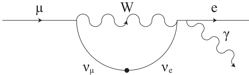
Figure 2.10: \mu \rightarrow e\gamma , as a Standard Model process. The black dot represents the conversion of the muon neutrino to an electron neutrino, in the Standard Model this process has a predicted branching ratio \sim < 10^{-54} and has not been seen.
