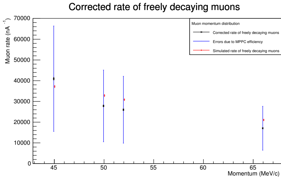
Figure 4.25: Corrected free muon decay rate and simulated free muon decay rate. The red lines are the simulated results, the blue lines the measured results including the MPPC efficiency error and the black lines are the measured values without the MPPC efficiency error.
