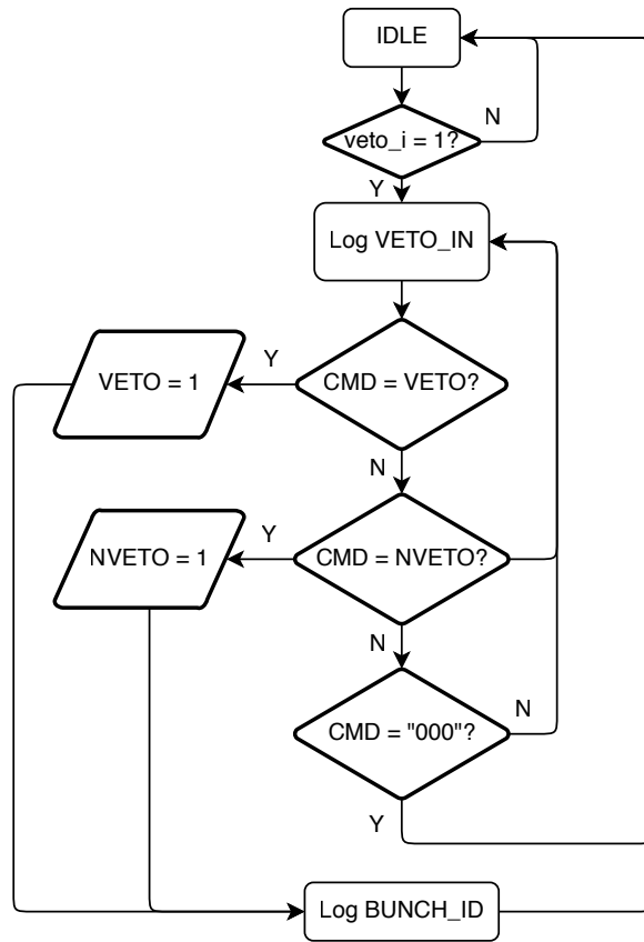
Figure 7.4: Flow diagram of the veto receiver entity. This de-serialises and splits the veto signals into the command and its payload, the Bunch ID. Note that this system also has the same flaw as the command receiver, i.e. it doesn't count bits as they are received so it can enter an undefined state if a malformed veto signal is sent.
