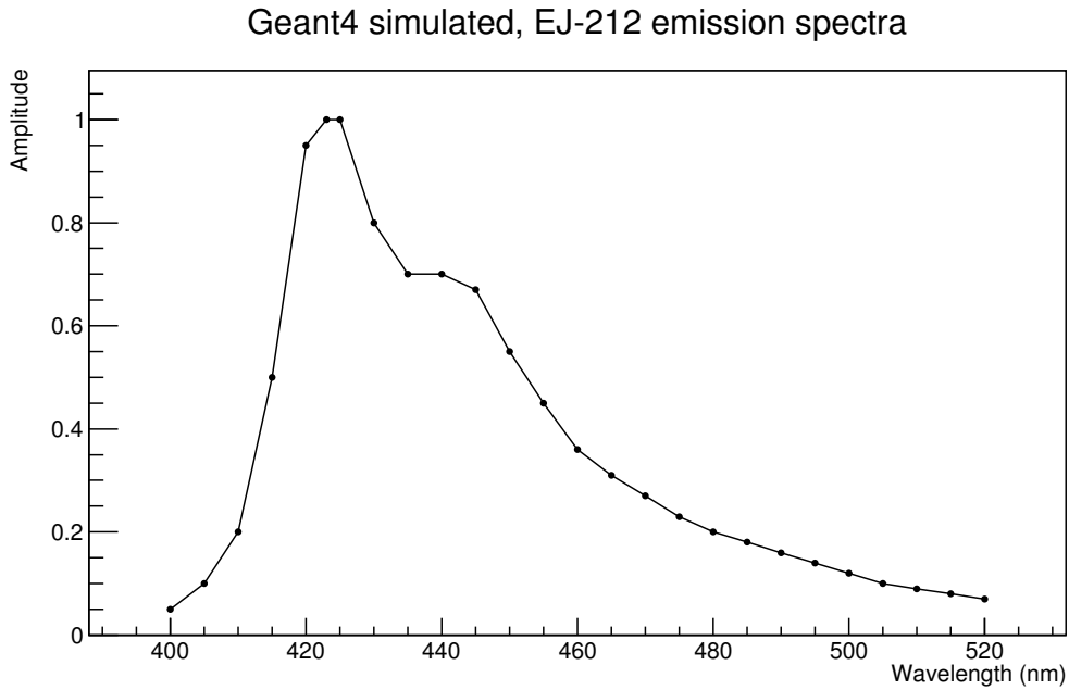
Figure 3.8: Scintillation spectra for EJ-212. The points represent the values passed to Geant4 and are based on those read from the manufacturer's data-sheet [27].
