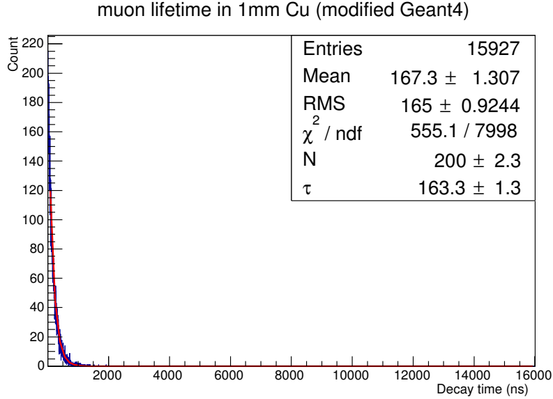
Figure 3.11: Decay time spectrum of 1 \times 10^6 negative muons hitting a 1 mm copper stopping target in a vacuum using a version of Geant4 modified to use the experimental muonic copper lifetime of 163.5 ns. The spectrum is fitted using N \exp(-x/\tau) . Only the muonic lifetime in copper is fitted as the decays are dominated by captured muons.
