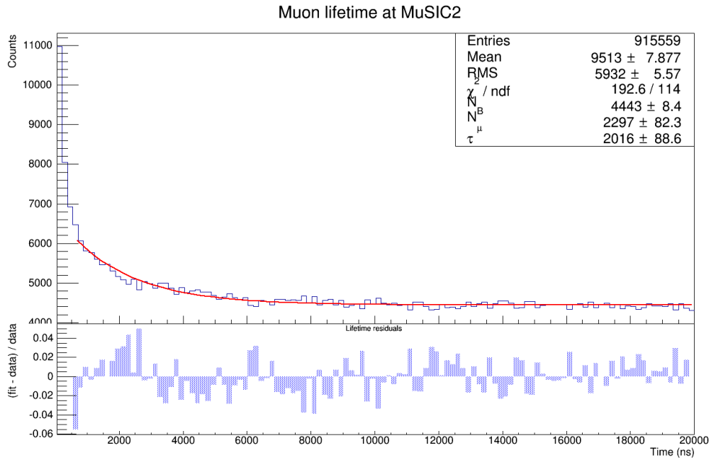
Figure 4.10: Results of the first measurement of the muon lifetime with residuals from the fit in the lower plot. The data was binned in 166 ns bins to remove the effects of noise on the data, only entries with an ADC value of 1,100 (which excluded the pedestal) were used. The fit was applied from 600 ns to 20 \mu s. The residuals show that fit gets worse at earlier times although this is to be expected with an exponential. Fitting with two exponentials should have improved the fit at earlier times but this was found not to be the case.
