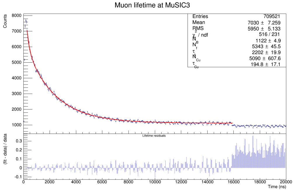
Figure 4.11: Results of the second measurement of the muon lifetime with residuals of the fit in the lower plot. The data was split between bins with a width of 50 ns and the data was fitted for values between 200 ns and 16 \mu\text{s} . The upper limit of the fit was lowered from 20 \mu\text{s} to 16 \mu\text{s} to remove an apparent discontinuity in the data. The discontinuity sits at 16 \mu\text{s} , and is especially clear in the residual plot. The cause of the discontinuity is unknown.
