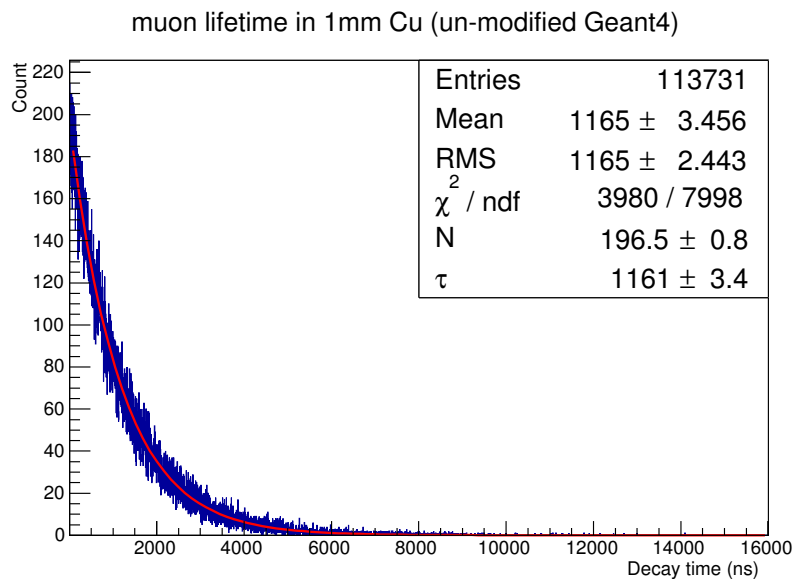
Figure 3.10: Decay time spectrum of 1 \times 10^6 negative muons hitting a 1 mm copper stopping target in a vacuum using an unmodified version of Geant4. The decay times are fitted using N \exp(-x/\tau) . As can be seen the Geant4 value, 1,161 ns, does not agree with either the experimentally determined value of 163.5 ns [3] or the theoretical value of 194 ns (calculated using the equation 2.6). This bug has been fixed in more recent versions of Geant4 (versions > 4.9.6 patch 02). Only the muonic lifetime in copper is fitted as the decays are dominated by captured muons.
