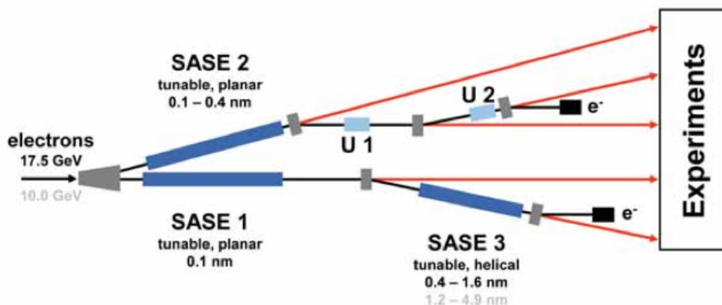
Figure 5.1: Schematic of the beam-lines for EuXFEL, black denotes electrons whilst red corresponds to X-rays. The blue ‘SASE’ blocks are SASE sections whilst the ‘U’ blocks are spontaneous emission undulators (which don’t self-amplify). Taken from [33].
