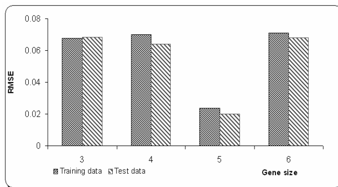
Figure 15: GEP leakage current approximation error for different gene sizes
