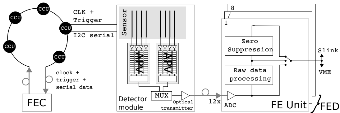
Figure 1. Scheme of the Data Acquisition System.
