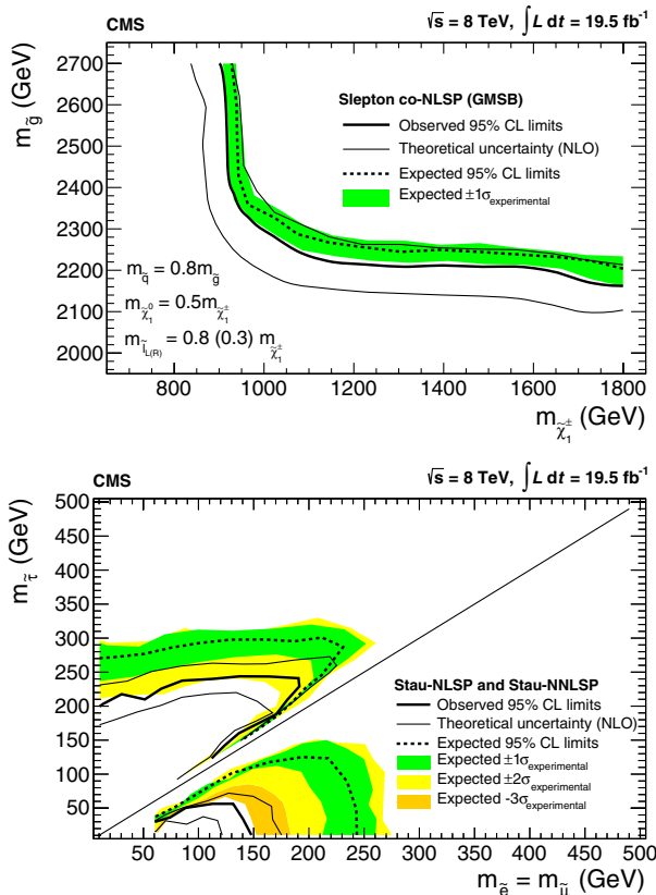
FIG. 8 (color online). The 95% confidence level upper limits for the slepton co-NLSP model in the gluino versus chargino mass plane (top) and for the stau(N)NLSP scenarios in the stau versus degenerate-smuon and -selectron mass plane (bottom). The region to the left and below the contours is excluded.
