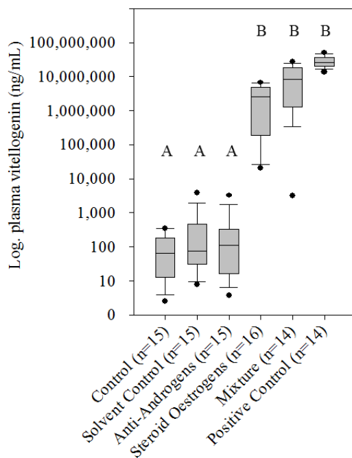
Figure 1. Log. Vitellogenin concentrations in the blood plasma of fathead minnow from each treatment group. Vitellogenin was not quantified in some cases when values were outside of the working range of the assay ( N number of samples is indicated out of 16 fish). Boxes represent the median with 25 th and 75 th percentiles and error bars extending to the 95 th percentile with outliers shown as dots. The labels A and B denote a statistically significant difference between groups at p \leq 0.05 .
