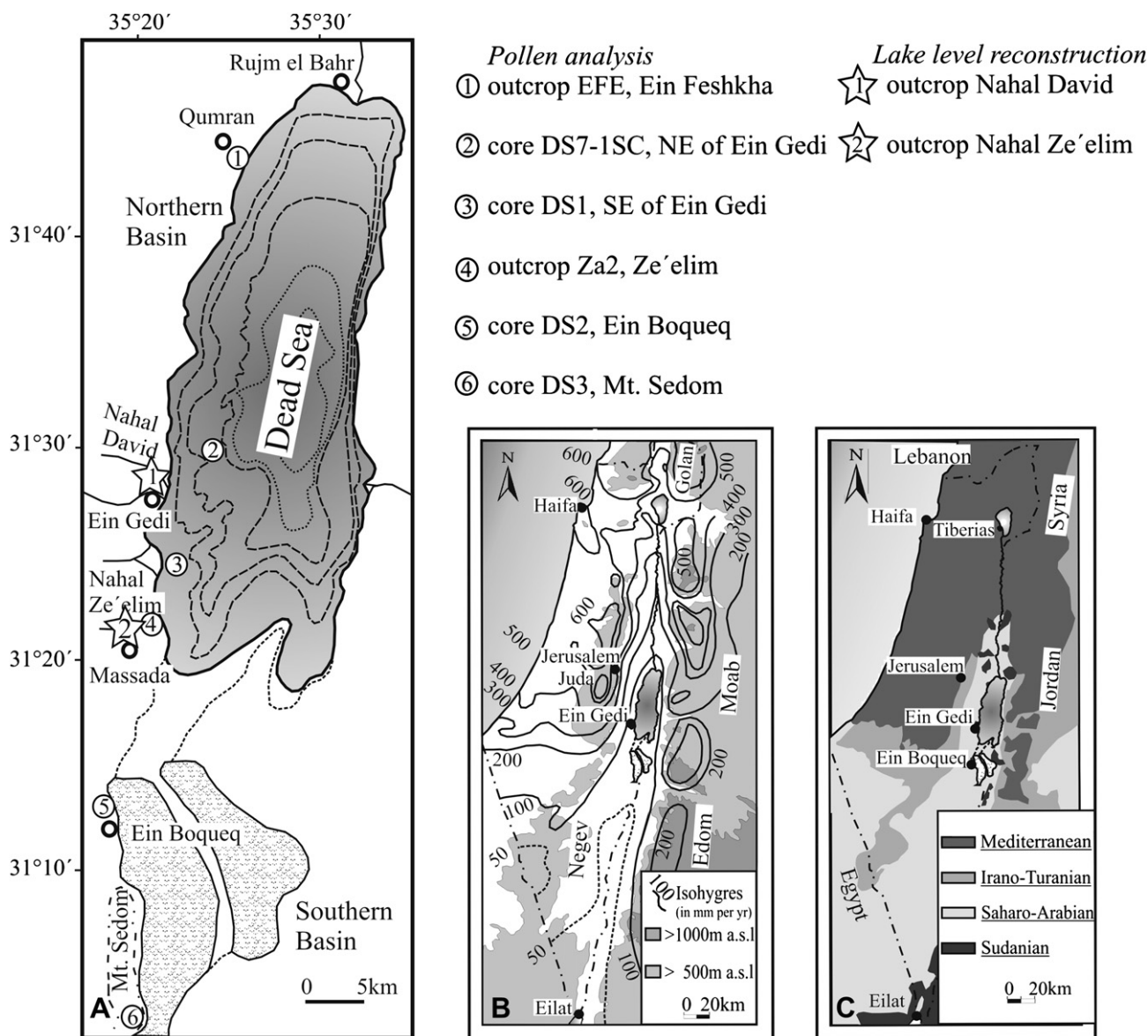
Fig. 1. A: Map of the Dead Sea showing the location of the cores and outcrops used for palynological and sedimentological research and discussed in this paper (after Baruch, 1990, 1993; Bookman (Ken-Tor) et al., 2004; Heim et al., 1997; Neumann et al., 2007). B: Topographical map of Israel and adjacent areas, black lines: annual rainfall contour lines in mm/year (after Jaffe, 1988). C: Plant geographical territories of Israel and adjacent areas (after Danin, 1988).
