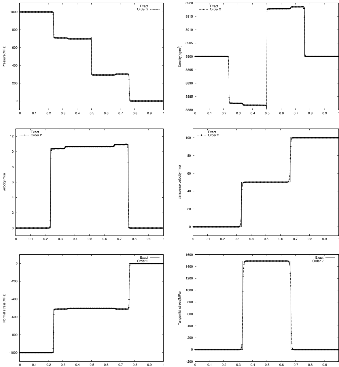
Figure 3: Results at t = 5 \cdot 10^{-5} for the solid-solid shock tube with copper in presence of a tangential velocity. Symbols represent our sharp interface method at second order with minmod slope limiter.
