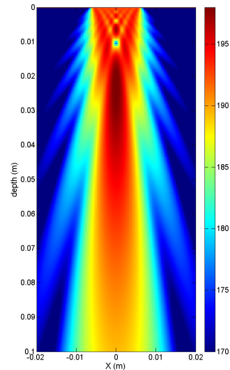
Figure 5: Theoretical pressure field (dB ref 1 \mu\text{Pa} ) for the primary frequency at 0.86 MHz.
