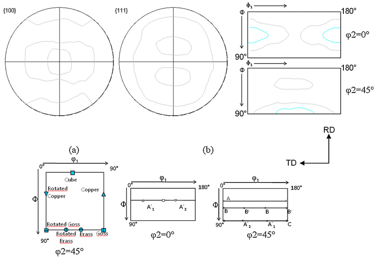
Fig. 5. Initial texture represented by the {100}{111} recalculated pole figures and \phi_2 = 0^\circ - \phi_2 = 45^\circ ODF sections. Levels: 1-2-3-4-5-6-7-8-9-10. The stable orientations are also indicated for the tensile tests (a) and for the shear test (b).
