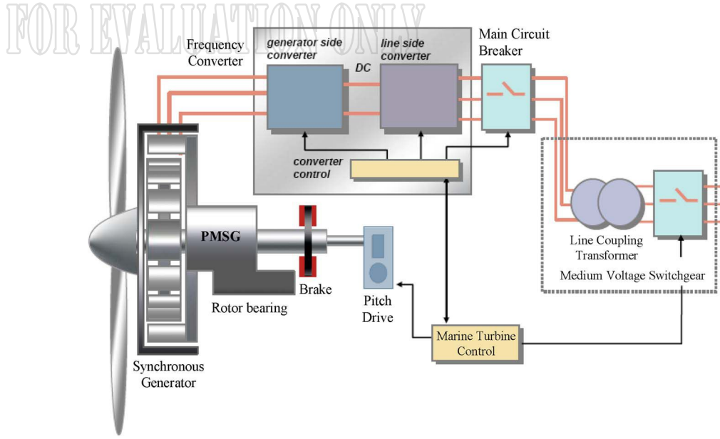
Fig. 4. Schematic diagram of a PMSG-based generation system.
