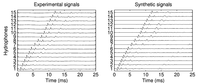
Fig. 4. Experimental (left) and synthetic (right) signals obtained for Site 2 at long range (700 m). The time origin is arbitrary.
