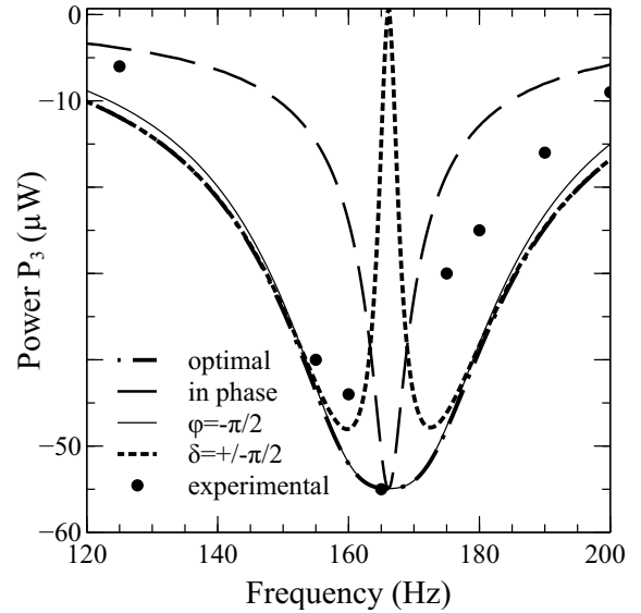
Figure 16: Electric power P_3 for \Gamma = 2m/sec^2 , as a function of the frequency f = \frac{\omega}{2\pi} ; \cdots optimal operating conditions; \cdots In-phase strategy, \cdots Maximal mechanical power strategy, \cdots Lower voltage strategy, \bullet : experimental.
