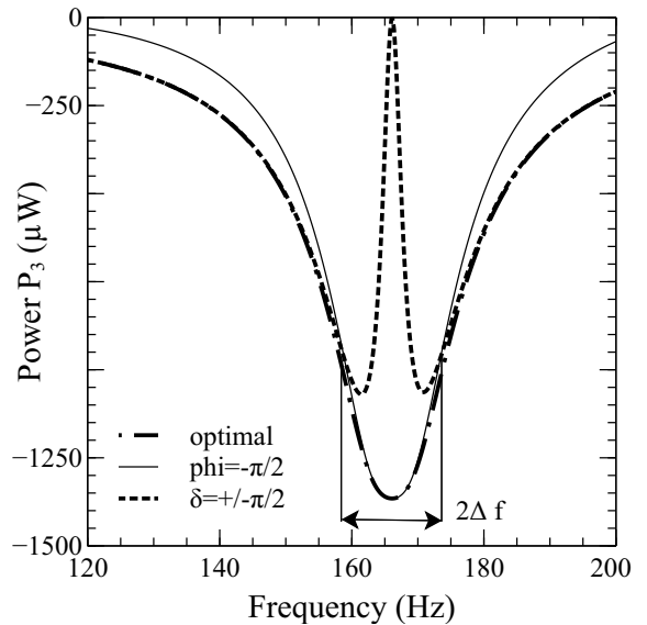
Figure 17: Electric power P_3 for \Gamma = 10m/sec^2 , as a function of the frequency f = \frac{\omega}{2\pi} ; \cdots optimal operating conditions; \cdots optimal mechanical power strategy, \cdots Lower voltage strategy.
