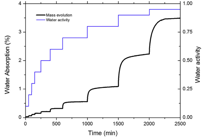
Fig. 5. Water absorption in 100 \mu\text{m} thick film for several water activities at 40 °C.
