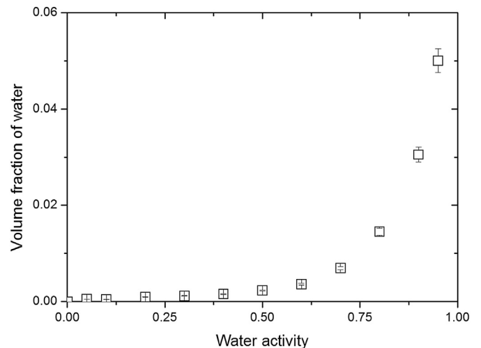
Fig. 6. Volume fraction of water in 100 \mu\text{m} CR film at 40 °C for different water activities.
