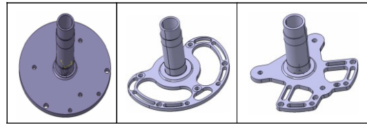
Figure 2: Various proposed design for forward steering part with combination of disk and tube shape [LC1].
