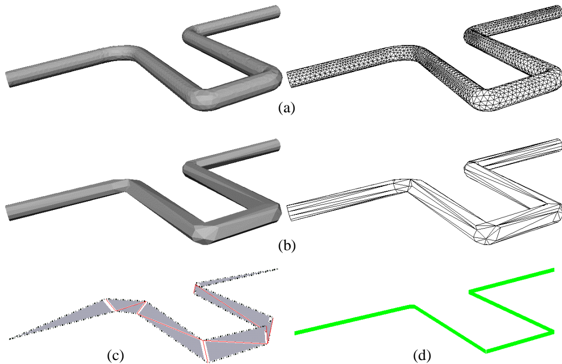
Figure 19 : Idealization process of a pipe : (a) initial polyhedron, (b) simplified model at \pm 0.01\text{mm} and without topological changes, (c) idealized geometry produce using only the vertex removal operators with topological changes, (d) final idealized geometry produced using the complementary operators proposed (i.e. the edge collapse operator in this example).
