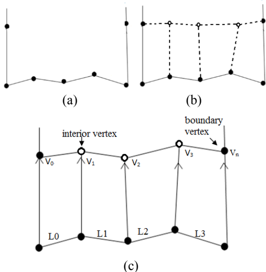
Figure 10 (a)A part of a cycle to be filled; (b) Connectivity constructed in the cycle; (c) Calculation of positions of interior vertices. Solid points are the boundary vertices and hollow points are the interior vertices
