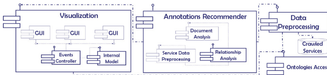
FIGURE 10.2: SWEET Architecture
