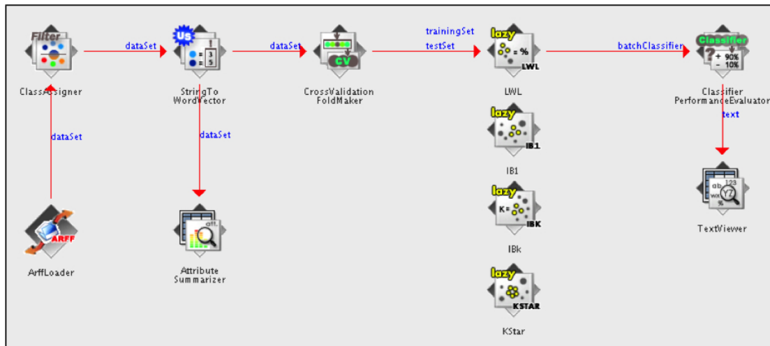
FIGURE 10.10: Classification Workflow
