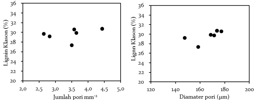
Gambar 4. Korelasi kadar lignin dengan jumlah dan diameter pori pada kayu tarik mindi. Figure 4. Correlation between lignin content with vessel number and diameter in tension wood of mindi.
