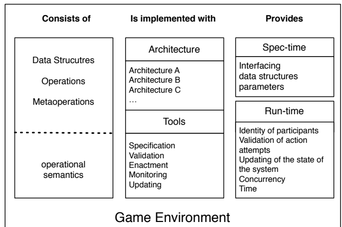
Figure 2. Game Environment
