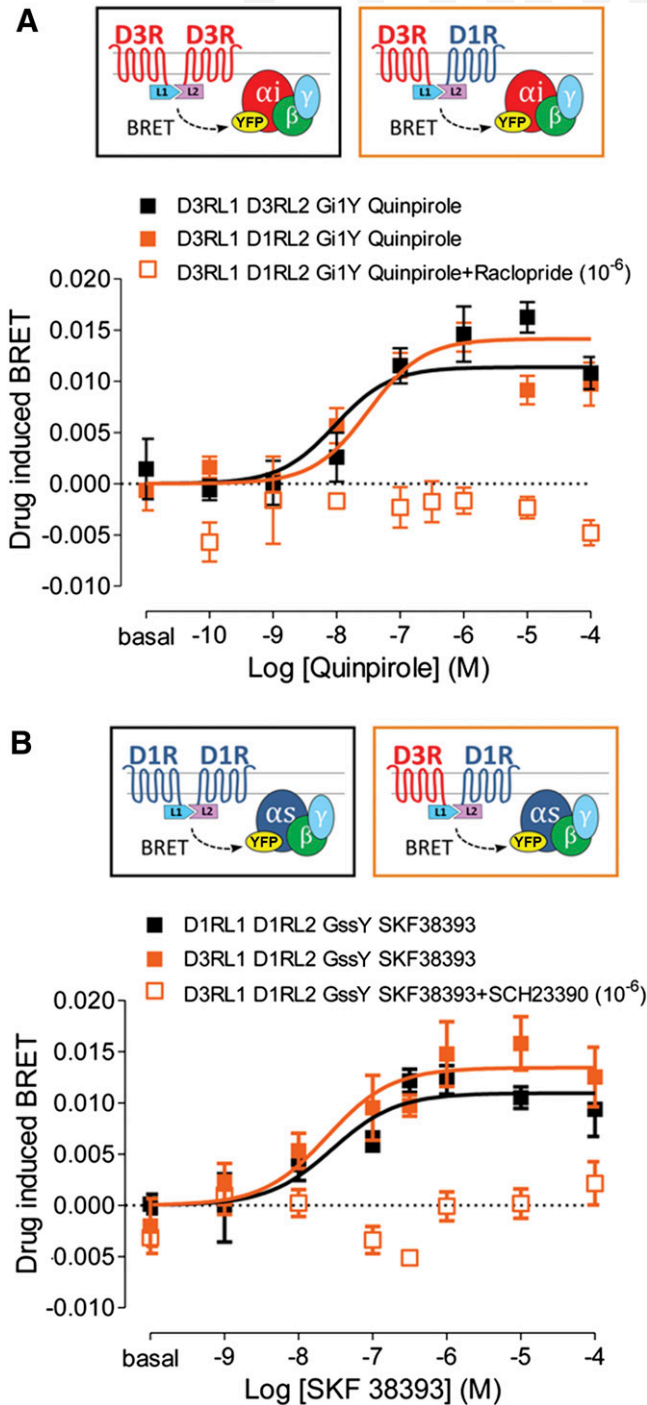
Fig. 1. G_s and G_i protein coupling to D1R-D3R heteromer determined by CODA-RET experiments. BRET between complemented hemitruncated Rluc (L1 and L2 are the N-terminal and the C-terminal domains of Rluc, respectively) and G protein-YFP, as indicated in the cartoons at the top, was determined in HEK-293 cells expressing the following: (A) G_{\alpha i1} -YFP (Gi1Y), D3R-L1 and D3R-L2 (black symbols), or D1R-L2 (orange symbols) or (B) G_{\alpha oss} -YFP (GssY), D1R-L2 and D1R-L1 (black symbols), or D3R-L1 (orange symbols). Cells were preincubated for 15 minutes at room temperature with medium (filled symbols) or with 1 \mu\text{M} D3R antagonist raclopride (A, orange open symbol) or the D1R antagonist SCH 23390 (B, orange open symbol) before the addition of increasing concentrations of D3R agonist quinpirole (A) or D1R agonist SKF 38393 (B). To the BRET values for each agonist concentration was subtracted the BRET value in the absence of ligands. Values are means \pm S.E.M. ( n = 3-5 ).
