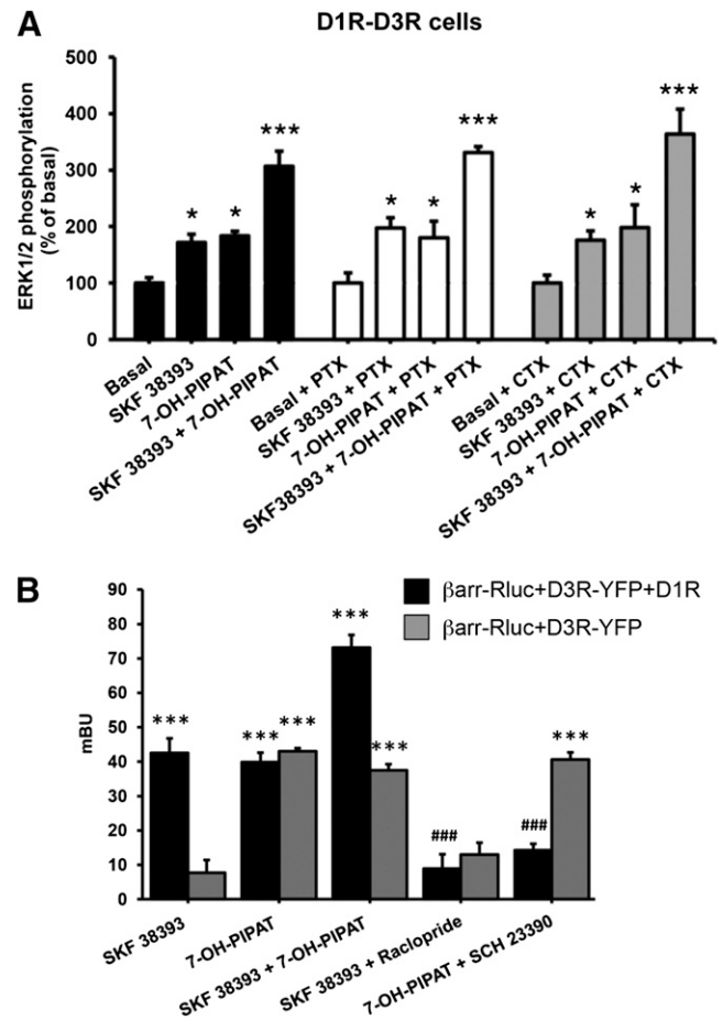
Fig. 9. G protein-independent mechanisms of the allosteric modulations in the D1R-D3R heteromer. (A) D1R-D3R cells were treated overnight with vehicle (black columns), with 10 ng/ml pertussis toxin (PTX, white columns), or with 100 ng/ml cholera toxin (CTX, gray columns). Cells were not stimulated (basal) or stimulated with 0.1 \mu M D1R agonist SKF 38393 or the D3R agonist 7-OH-PIPAT alone or in combination. Values are expressed as percentage over basal and are means \pm S.E.M. ( n = 5 ). (B) HEK-293T cells were transfected with the cDNA corresponding to D3R-YFP (1 \mu g cDNA) and \beta -arrestin-1-Rluc (0.5 \mu g cDNA) in the absence (gray columns) or presence of D1R (1.5 \mu g cDNA) (black columns). Forty-eight hours post-transfection, cells were treated with vehicle or 1 \mu M D3R antagonist raclopride or the D1R antagonist SCH23390 before stimulation with 0.1 \mu M 7-OH-PIPAT or SKF 38393, and \beta -arrestin-1 recruitment was measured by BRET experiments. Values are means \pm S.E.M. ( n = 7-8 ). Significant differences were calculated by one-way analysis of variance with post hoc Newman-Keuls test: * P < 0.05 , *** P < 0.001 versus basal values; (B) ### P < 0.001 as compared with agonist alone.
