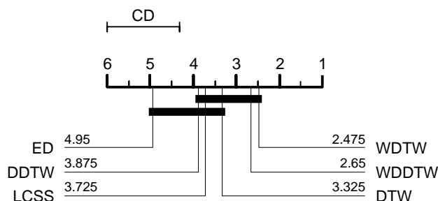
Fig. 6. The average ranks for 1-NN classifiers for Euclidean Distance (ED), Longest Common Subsequence (LCSS), Dynamic Time Warping (DTW), Derivative Dynamic Time Warping (DDTW), Dynamic Time Warping with window set through cross validation (DTWCV) and weighted versions (WDTW and WDDTW) for 20 data sets. Data taken directly from [8].
