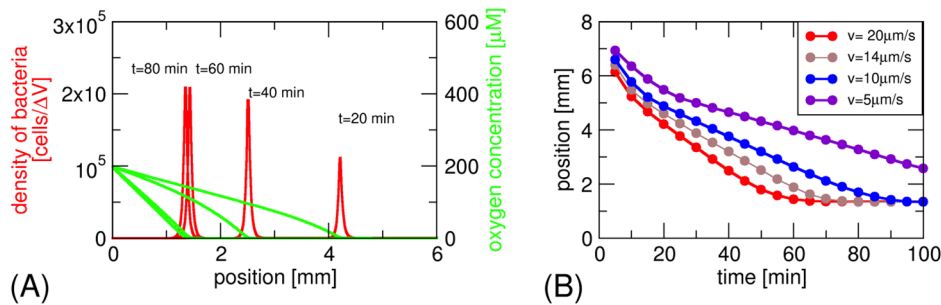
Figure 3. Formation of the aerotactic band in a model for magneto-aerotaxis: (a) Density profile of the bacteria (sharp band, shown in red) and of the oxygen concentration (green) at different time points. The parameter values for the simulations are as given in Table S1, corresponding to a magnetic field parallel to the oxygen gradient. Bacterial densities are given in number of cells per discretization volume \Delta V (see Table S1). (b) Position of the aerotactic band as a function of time for different bacterial swimming speeds. A magnetic field at an angle to the oxygen gradient can be interpreted as effectively reducing the swimming speed in the direction of the gradient (the projected swimming speed). Under this simplifying assumption the four speed values correspond to angles of 0^\circ , 45^\circ , 60^\circ , and 75^\circ . doi:10.1371/journal.pone.0101150.g003
