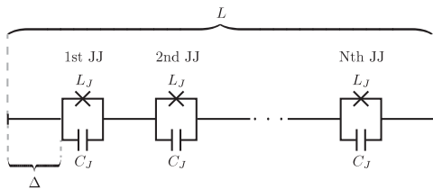
FIG. 1. Central conductor of a CPWR of length L interrupted by N identical and uniformly distributed JJ with Josephson inductance L_J and capacitance C_J .
