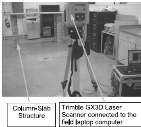
Figure 3: Experimental setup
