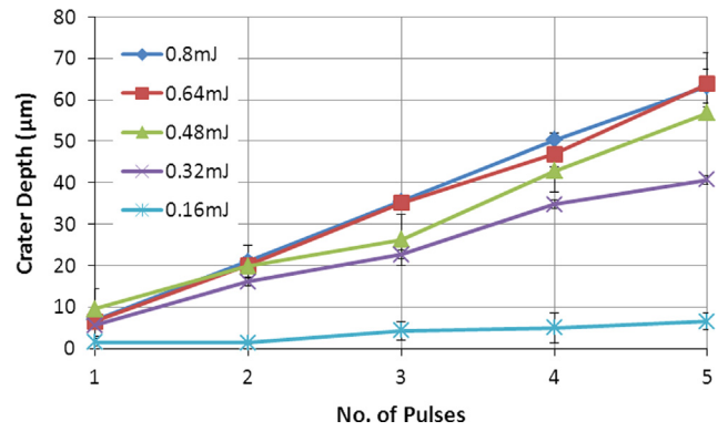
Fig. 4. Crater depth as a function of number of pulses for different pulse energies.
