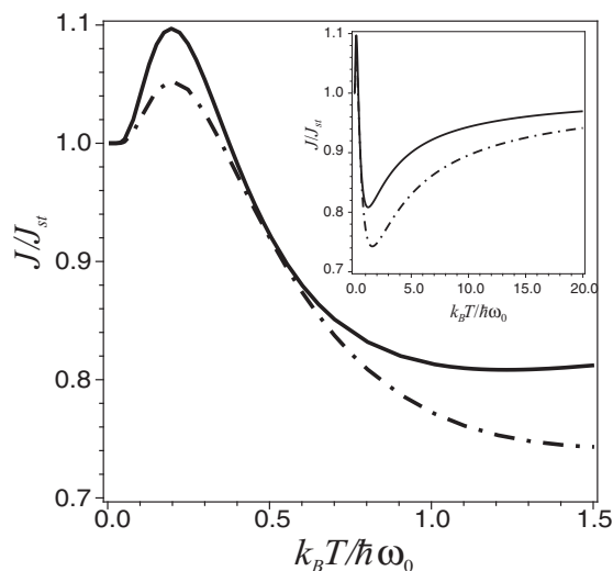
FIG. 3. Temperature dependence of the ratio between the critical Josephson current and the "standard" result for the critical current, J_{st} = (e\Gamma_0^2/2\hbar\tilde{\varepsilon}) \tanh(\tilde{\varepsilon}/2T) . In each case (solid curve: g = 1.4 , dash-dotted curve: g = 2.0 ) \tilde{\varepsilon} was chosen to make the ratio unity at T = 0 . Deviations from unity at low and intermediate temperatures indicate an anomalous temperature dependence of the Josephson current. The plotted ratio approaches unity (from below) only asymptotically at high temperatures (see inset).
