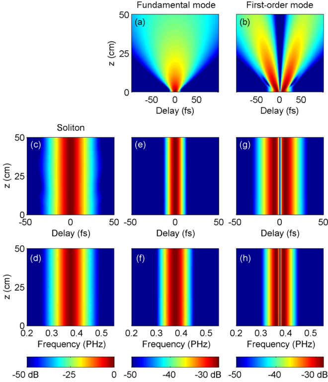
FIG. 1. (Color online) (a), (b) Propagation of a dispersive radiation solely in an argon-filled HC-PCF, when the radiation takes the form of (a) the fundamental mode f_0(\tau) , or (b) the first-order mode f_1(\tau) . (c)–(h) Propagation of a fundamental soliton and a dispersive radiation together in an argon-filled HC-PCF. The group-velocity matching condition is satisfied. The two pulses have the same central wavelength \lambda = 800 nm, and opposite circular polarizations. (c), (d) Temporal and spectral evolution of the radiation, when it is in the fundamental mode [(e),(f)], or in the first-order mode [(g),(h)]. Other simulation parameters are \eta = 8.9 , \psi_0 = 0.5 , and t_0 = 50 fs. The higher-order dispersion and self-steepening effects are neglected.
