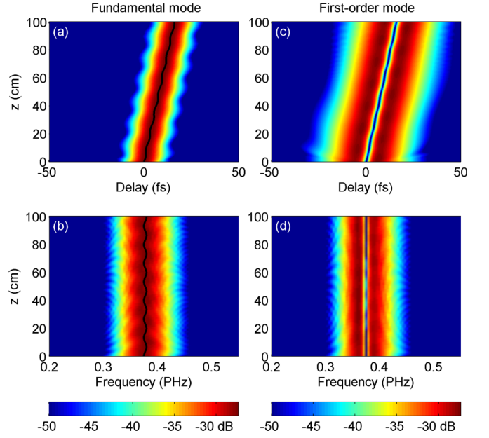
FIG. 2. (Color online) Propagation of a fundamental soliton and a dispersive radiation in an argon-filled HC-PCF in the presence of the self-steepening effect. Other simulation parameters are similar to those used in Fig. 1. Temporal and spectral evolution of the radiation, when it is in the fundamental mode [(a),(b)], or in the first-order mode [(c),(d)], respectively. Solid black lines are the numerical solutions of the coupled differential equations (7).
