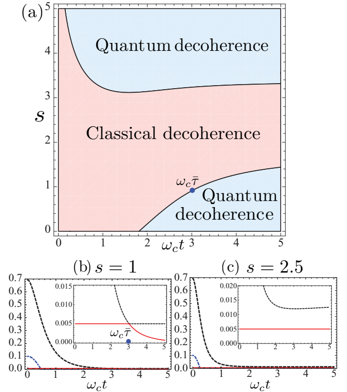
FIG. 1. (Color online) (a) Landscape of correlation dynamics in the s - t plane, for c = 0.1 and T = 0 . Blue (dark gray) areas denote parameters (t, s) corresponding to quantum decoherence, red (gray) areas to classical decoherence and the intersection between the two, marking the values of s and \bar{t} satisfying Eq. (9), which defines the transition time \bar{t} as a function of the reservoir spectrum parameter s . The smaller figures show discord (solid red line), classical correlations (dashed black line), and entanglement measured by concurrence [27] (dotted-dashed blue line) for two specific choices of s ; (b) for s = 1 the system has a sudden transition from quantum to classical decoherence while for (c) s = 2.5 the discord is frozen forever. The blue (dark gray) dot in (a) and (b) points the transition time \bar{t} for s = 1 .
