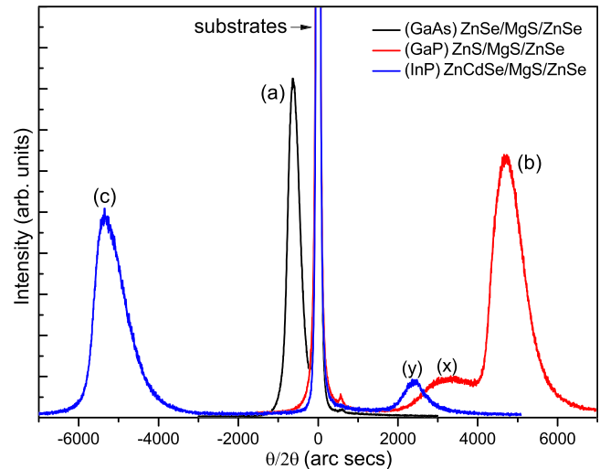
FIG. 2. XRD rocking curves from (a) GaAs/ZnSe/MgS/ZnSe, (b) GaP/ZnS/MgS/ZnSe, and (c) InP/ZnCdSe/MgS/ZnSe structures. Peaks from the three substrates have been aligned at the origin. Peaks (a), (b), and (c) are from the ZnSe cap layers for these three structures, whereas (x) and (y) peaks originate from ZnS and ZnCdSe buffer layers, respectively.
